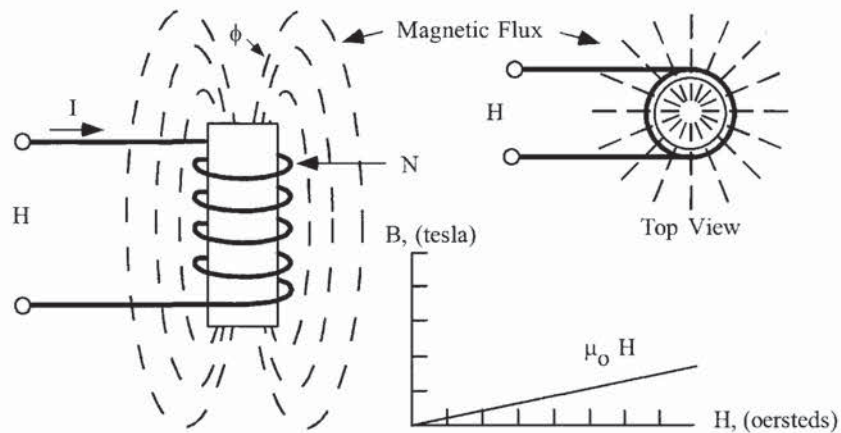
Figure 1-10. Air-Core Coil Emitting Magnetic Flux when Excited.
