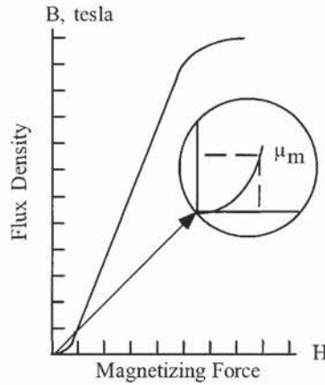
Figure 1-24. Material Permeability.
