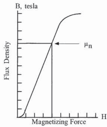
Figure 1-22. Normal Permeability.
