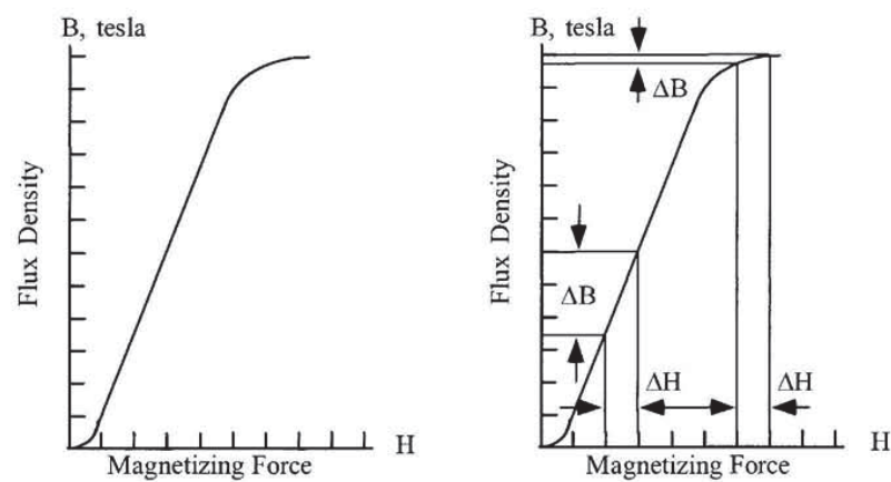
Figure 1-18. Magnetizing Curve.
