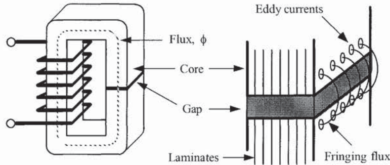
Figure 1-33. Fringing Flux, with High Loss Eddy Currents.
