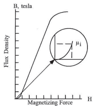
Figure 1-20. Initial Permeability.
