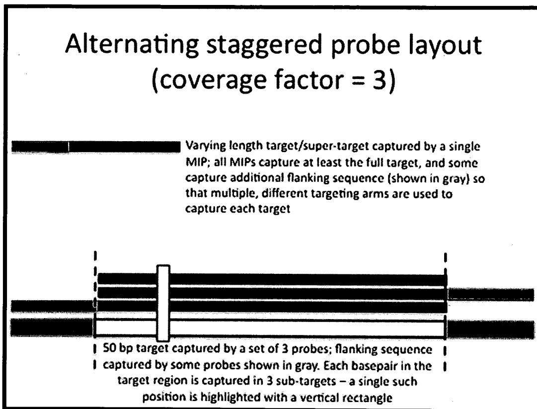
Figure 3. Alternating staggered probe layout, showing the targets captured by a set of three MIPs. Each MIP captures the full target, shown in black, plus (in some cases) additional extra-target sequence, shown in gray, such that the targeting arms of each MIP fall on different sequence. Each position in the target is covered by three sub-targets such that MIP performance per basepair is averaged across three probes.
