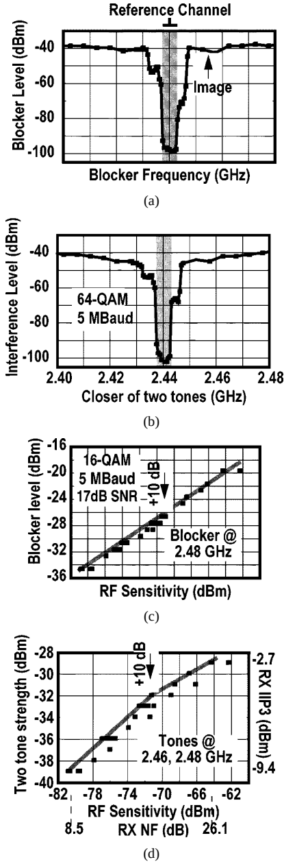
Fig. 20. Complete receiver measurements. (a) Single-tone blocker strength at various frequencies which desensitizes receiver by 3 dB. (b) Two-tone strength which desensitizes receiver by 3 dB because the intermodulation product lies on the reference channel. (c) Sensitivity versus blocker strength as the IF section adapts. (d) Sensitivity versus IIP3 as the IF section adapts to two in-band tones.
