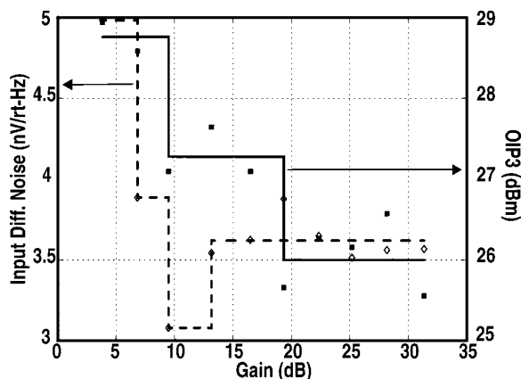
Fig. 14. Measured noise and output of IP3 of prefilter PGA (shown in Fig. 9) versus gain, when LPWstep is used.
