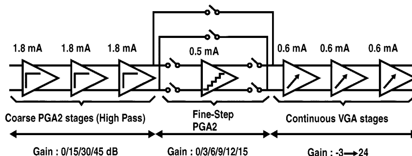
Fig. 13. Post-filter PGA2 with HPF, and VGA.
