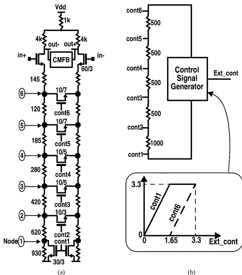
Fig. 11. (a) VGA circuit using soft-switched degeneration. (b) Resistor ladder and control voltages.
