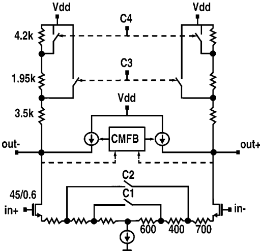
Fig. 8. Fine-step PGA, low-power version.
