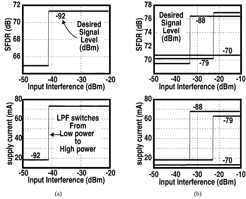
Fig. 18. Adapting dynamic range to levels of interferer and desired signal. (a) Desired signal at the minimum level. (b) At three levels of the desired signal.
