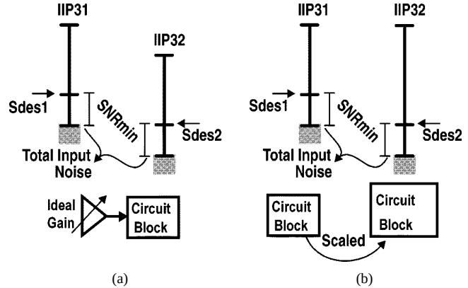
Fig. 4. An illustration of how to achieve: (a) slide DR with preamplification and (b) step DR by substitution of a scaled circuit block.
