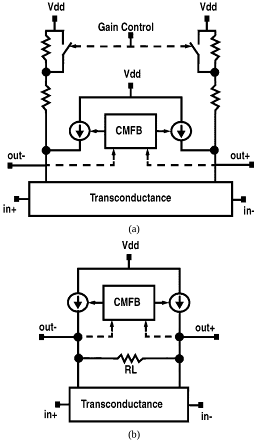
Fig. 7. Biasing alternatives with resistor loads. (a) RL connected to supply. A small part of current is supplied by the current sources. (b) Floating load resistor. All bias current is supplied by the current sources.
