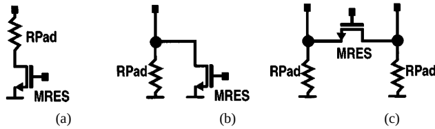
Fig. 10. Illustrating degeneration by: (a) serial resistor padding, (b) parallel padding and (c) parallel differential padding.
