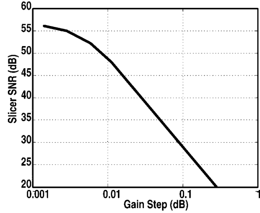
Fig. 5. Detected SNR of 64-QAM bitstream as a function of a gain jump during reception.
