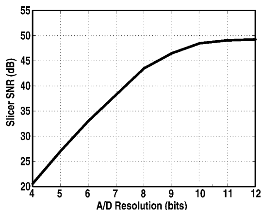
Fig. 12. Detected SNR of a 64-QAM signal versus A/D resolution, assuming signal loads A/D 90% at the peak.
