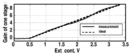
Fig. 15. Gain of one VGA stage versus control voltage.
