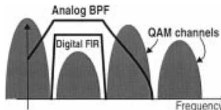
Fig. 1. Complete channel select filter is a combination of the analog BPF and a digital FIR filter.
