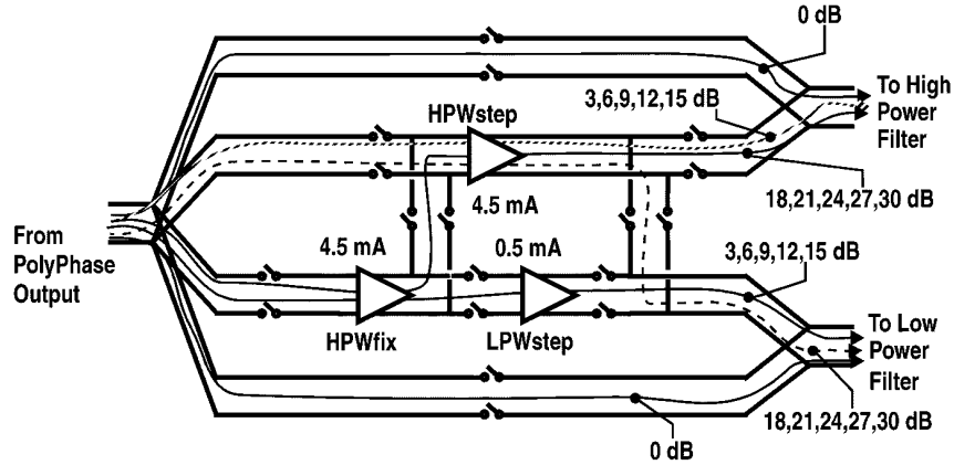
Fig. 9. Combination of PGA stages realizing PGA1.
