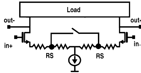
Fig. 6. Switched degeneration with a single tail current source. Voltage headroom limits loop gain.
