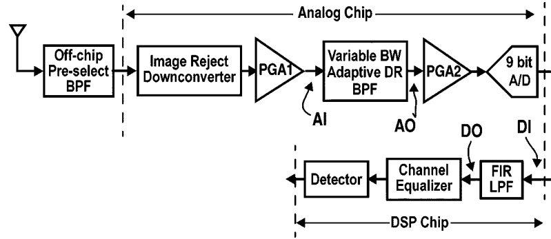
Fig. 2. Block diagram of complete WLAN receiver.
