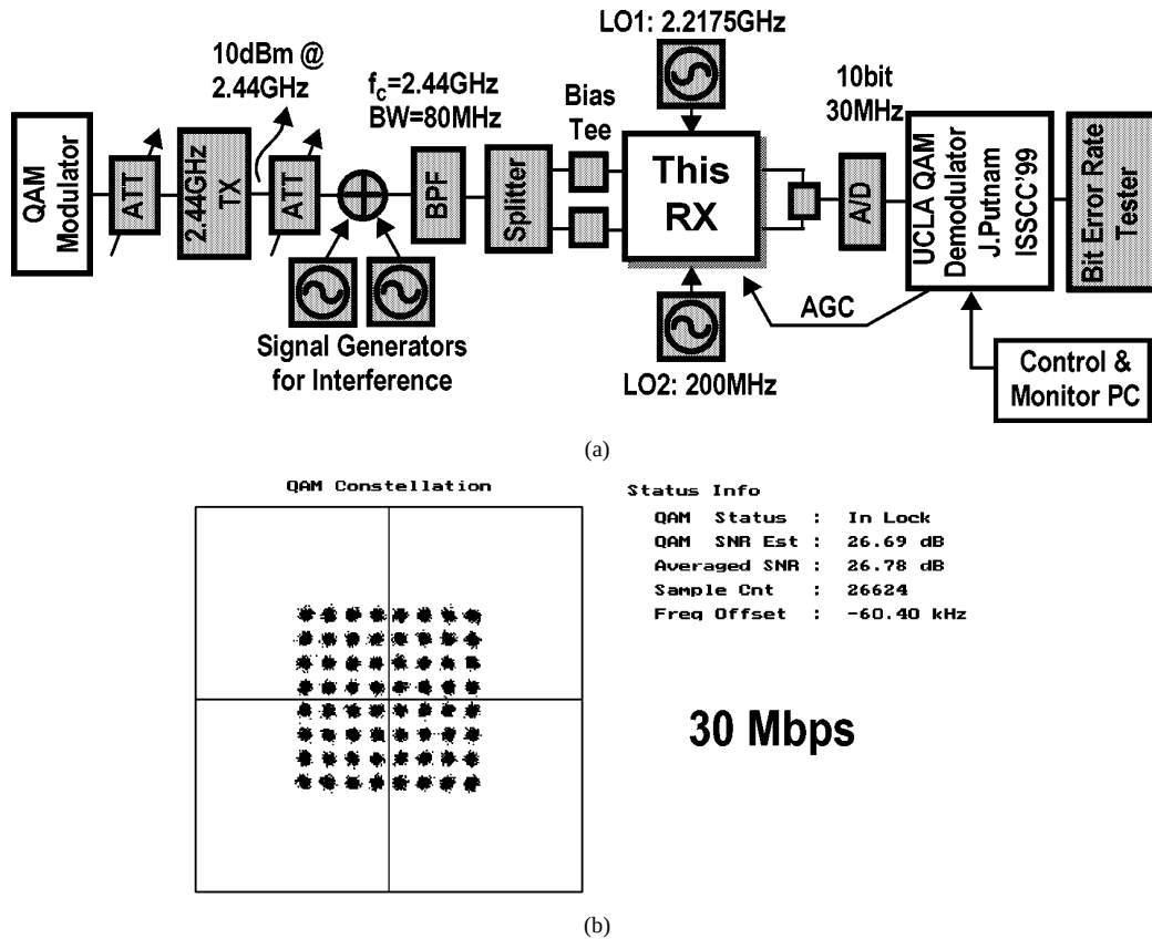
Fig. 19. (a) RX measurement setup. (b) Measured 64-QAM constellation at the baseband.
