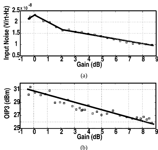
Fig. 16. (a) Noise and (b) output IP3 of one VGA stage versus gain.
