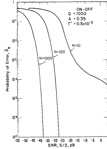
Figure 8. The upper bound on performance, \hat{P}_e , (26) for the ON-OFF signaling case for Q = 1000 and N = 10, 100 , and 1000 , the number of independent samples.
