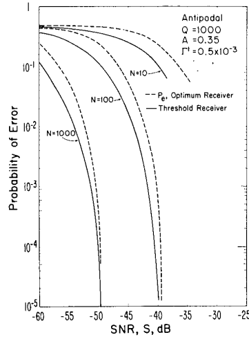
Figure 14. Comparison of the estimate of performance for small signal (42) with the upper bound on performance (26) for Q = 1000 , N = 10 , 100 , and 1000 for antipodal signals.
