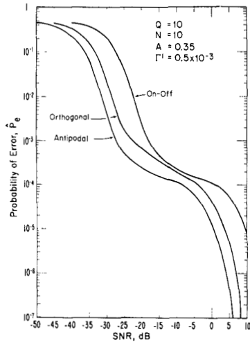
Figure 6. The upper bound on performance, \hat{P}_e , (26) for the three signaling cases (24) for N = 10 independent samples and Q = 10 .
