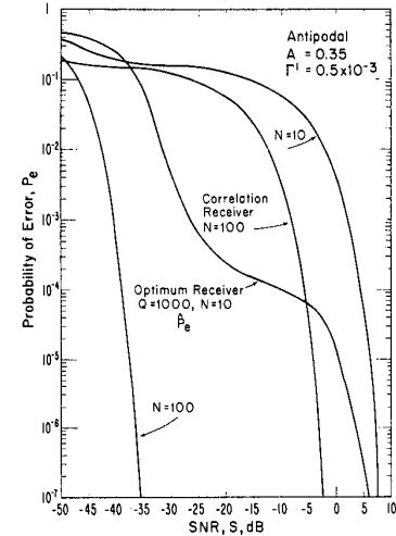
Figure 11. Comparison of performance of correlation receiver in Class A interference with the upper bound on optimum performance (26) for Q = 1000 and N = 10 and 100 for antipodal signals.
