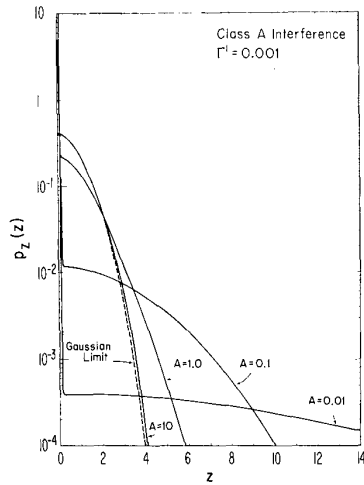
Figure 1. The pdf of the instantaneous amplitude of the interference z (Class A) for \Gamma' = 0.001 from (7).
