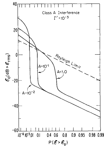
Figure 2. The envelope distribution [ \text{prob}(E > E_0) ] for Class A interference for \Gamma' = 10^{-3} and various A from (9).
