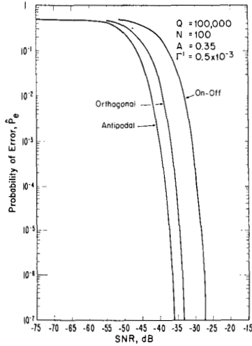
Figure 7. The upper bound on performance, \hat{P}_e , (26) for the three signaling cases (24) for N = 100 independent samples and Q = 100,000 .
