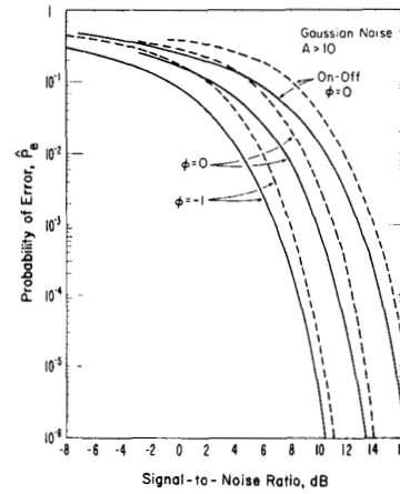
Figure 9. Comparison of theoretical performance in Gaussian noise (from (27)) and the upper bound (28) (dashed curves).
