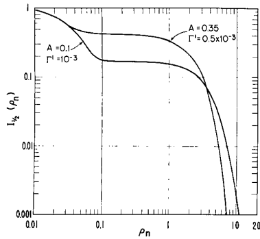
Figure 5. The integral I_{1/2}(\rho_n) , (21b) for two example cases along with the upper bound \hat{I}_{1/2}(\rho_n) , (25).
