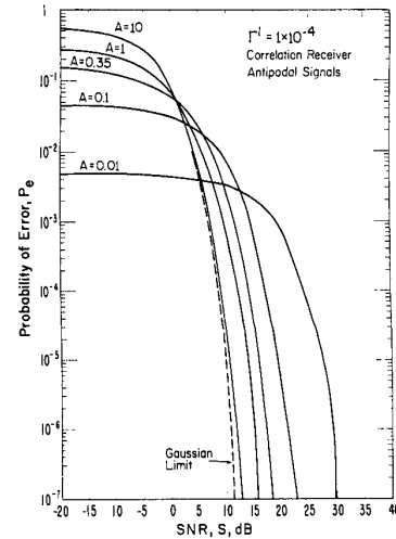
Figure 10. Performance of the correlation receiver (Gaussian optimum receiver) in Class A interference (30) for \Gamma' = 10^{-4} for various values of the impulsive index A .
