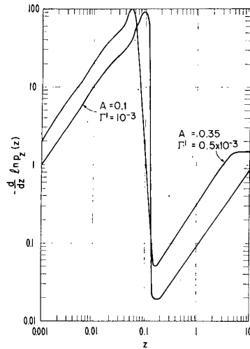
Figure 13. The nonlinearity, -d/dx \ln p_Z(z) , for two example cases of Class A interference.
