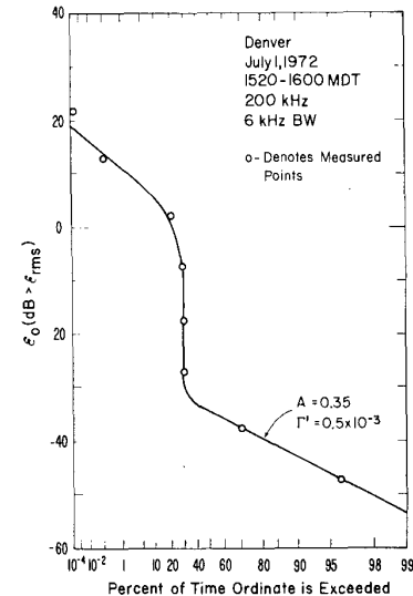
Figure 3. Comparison of measured envelope distribution (from Bolton [14], narrowband interference) with the Middleton model [4], Class A, distribution (9).
