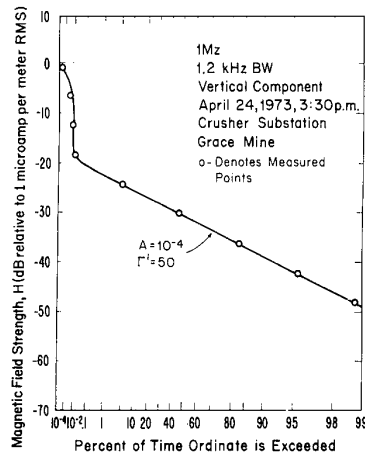
Figure 4. Comparison of measured envelope distribution (from Adams et al. [13], ore-crushing machinery) with the Middleton model [4], Class A, distribution (9).
