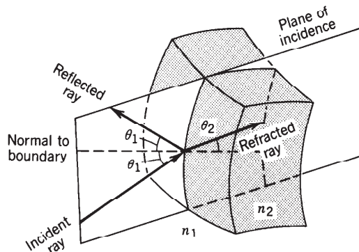
Figure 1.1-3 Reflection and refraction at the boundary between two media.
