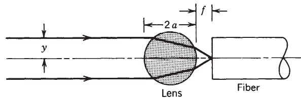
Figure P1.2-4 Focusing light into an optical fiber with a spherical glass ball.
