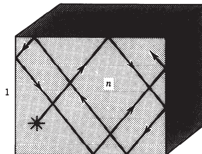
Figure 1.2-19 Trapping of light in a parallelepiped of high refractive index.
