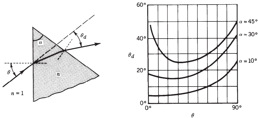
Figure 1.2-10 Ray deflection by a prism. The angle of deflection \theta_d as a function of the angle of incidence \theta for different apex angles \alpha when n = 1.5 . When both \alpha and \theta are small \theta_d \approx (n - 1)\alpha , which is approximately independent of \theta . When \alpha = 45^\circ and \theta = 0^\circ , total internal reflection occurs, as illustrated in Fig. 1.2-9(b).
