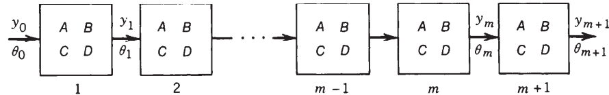
Figure 1.4-5 A cascade of identical optical components.
