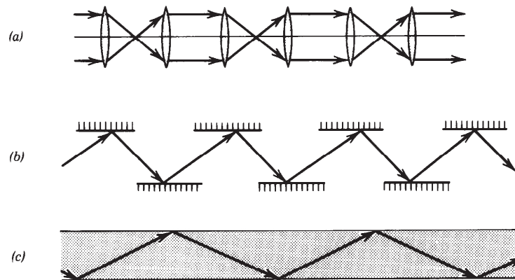
Figure 1.2-16 Guiding light: (a) lenses; (b) mirrors; (c) total internal reflection.
