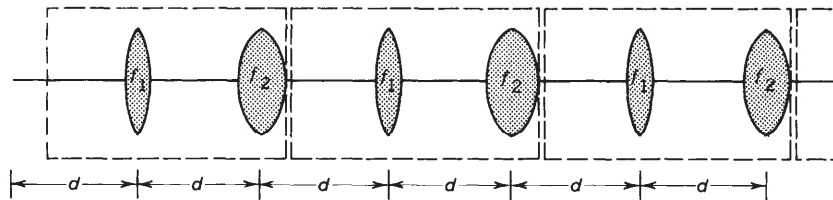
Figure 1.4-9 A periodic sequence of lens pairs.
