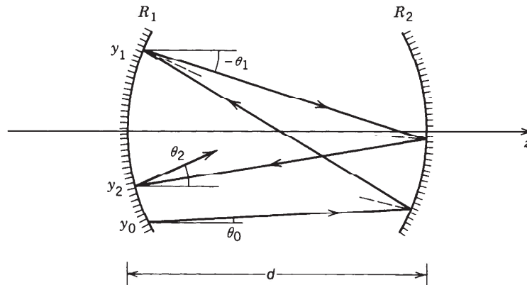
Figure 1.4-10 The optical resonator as a periodic optical system.
