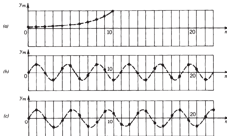
Figure 1.4-6 Examples of trajectories in periodic optical systems: (a) unstable trajectory ( b > 1 ); (b) stable and periodic trajectory ( \varphi = 6\pi/11 ; period = 11 stages); (c) stable but nonperiodic trajectory ( \varphi = 1.5 ).
