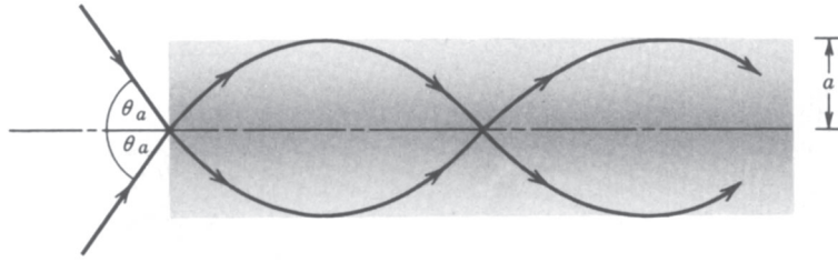
Figure 1.3-8 Acceptance angle of a graded-index optical fiber.
