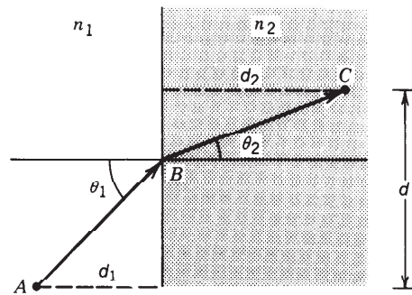
Figure 1.1-4 Construction to prove Snell's law.
