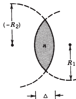
Figure 1.2-13 A biconvex spherical lens.
