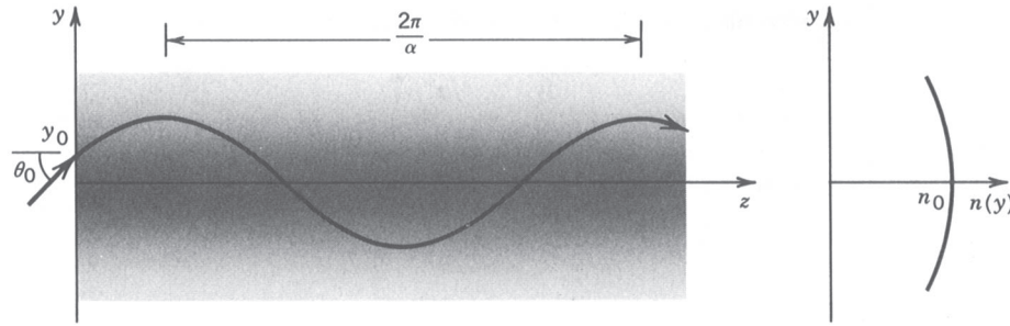
Figure 1.3-4 Trajectory of a ray in a GRIN slab of parabolic index profile (SELFOC).
