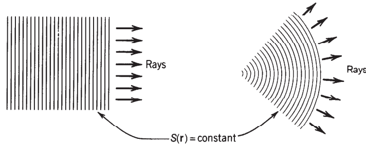
Figure 1.3-10 Rays and surfaces of constant S(\mathbf{r}) in a homogeneous medium.
