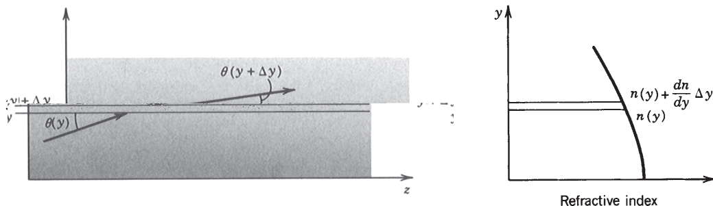
Figure 1.3-3 Refraction in a graded-index slab.
