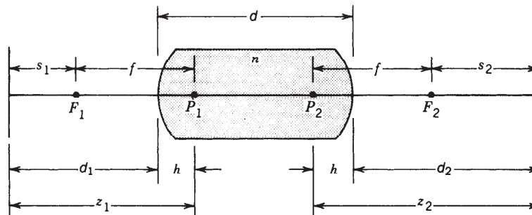
Figure 1.4-4 Imaging with a thick lens. P_1 and P_2 are the principal points and F_1 and F_2 are the focal points.
