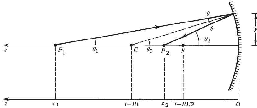
Figure 1.2-6 Reflection of paraxial rays from a concave spherical mirror of radius R < 0 .
