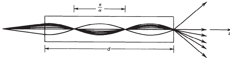
Figure 1.3-5 Trajectories of rays in a SELFOC slab.
