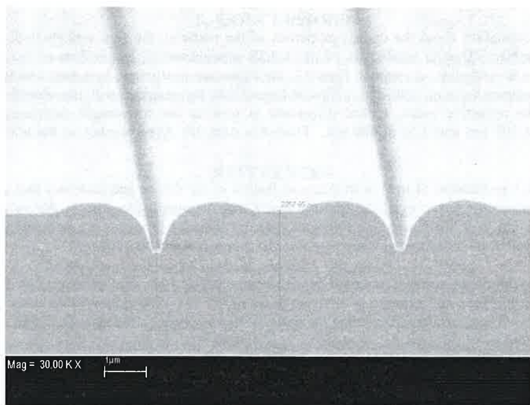
Figure 10. Cross-section SEM micrograph at 6- \mu m pitch (~93% feature density) on the wafer press-patterned for 120 seconds.
