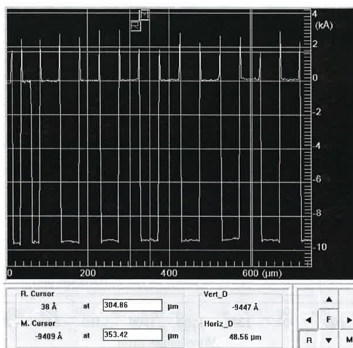
Figure 6. Step height profile of the SKW 7-2 test wafer in a 100-μm pitch size area.
