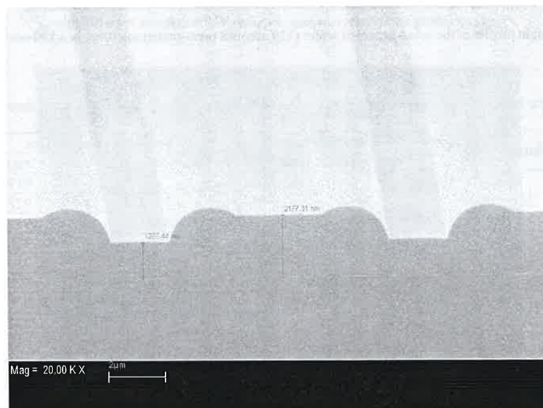
Figure 9. Cross-section SEM micrograph at 10- \mu m pitch (~75% feature density) on the wafer press-patterned for 120 seconds.
