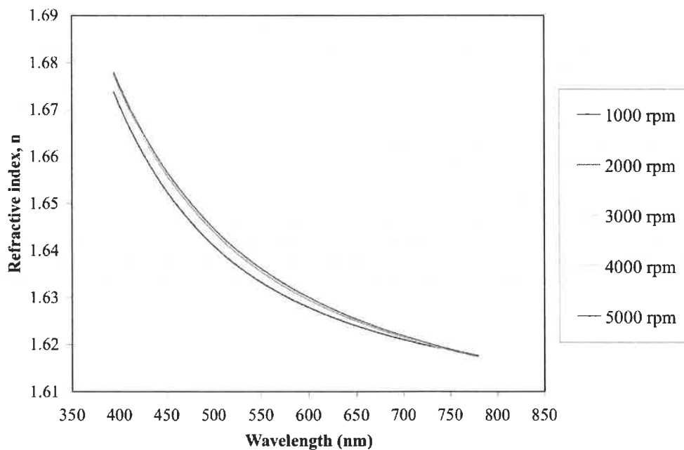
Figure 2. Extrapolated refractive index curves for the cured material coated on silicon wafers at various spin speeds.
