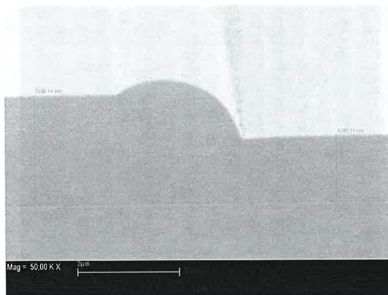
Figure 8. Cross-section SEM micrograph at 50- \mu m pitch (~55% feature density) on the wafer press-patterned for 120 seconds.
