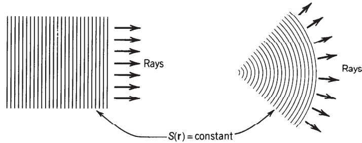
Figure 1.3-10 Rays and surfaces of constant S(\mathbf{r}) in a homogeneous medium.
