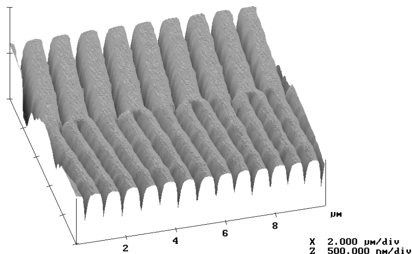
Figure 2. Grating structure of an Exelgram image viewed by Atomic Force Microscopy showing the change in spacing between two switch regions [4].
