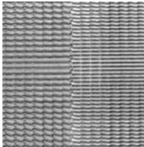
Figure 1. Optical microscope view of the grating structure of an Exelgram OVD image with a change in spatial frequency at the channel boundary.
