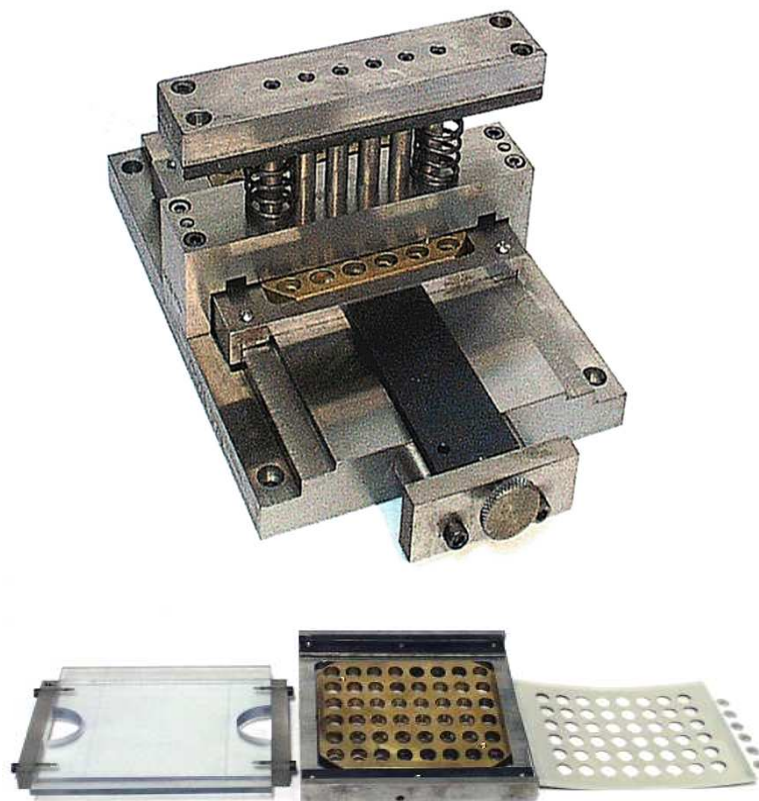
Fig. 7 Blanking tool (top), positioning aid (bottom left), nest (bottom centre) and cut shim
