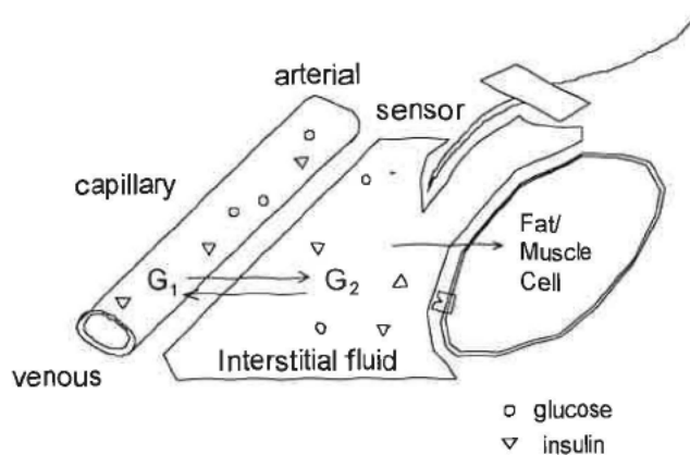
Figure 1. Glucose electrode inserted in subcutaneous tissue. Glucose diffuses from the intravascular compartment ( G_1 ) into the interstitial compartment ( G_2 ) and is then taken up by cells if insulin is present (modified after [11])
