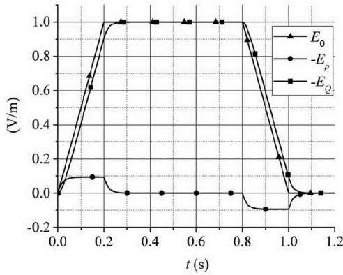
Fig. 2. Time evolution of the field due to external sources ( E_0 ) and of the fields due to bound and free charges ( E_p and E_Q , respectively). These latter are plotted with reversed sign to facilitate the comparison.
