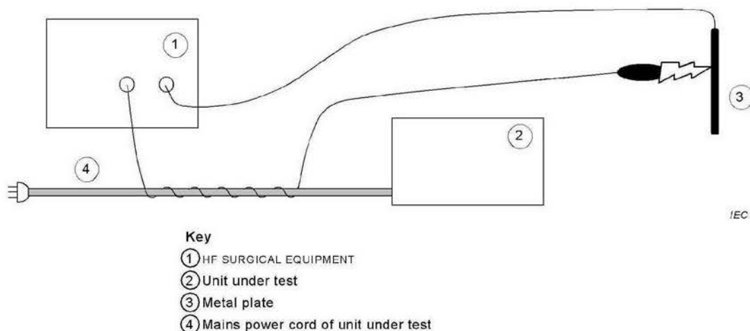
Figure BB.5 – Power cord ad hoc test
