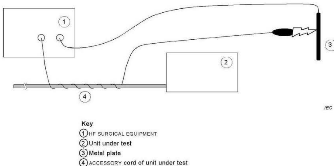
Figure BB.6 – ACCESSORY cord ad hoc test
