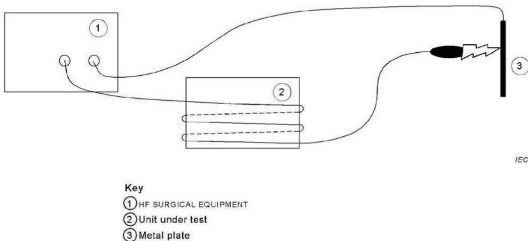
Figure BB.4 – Unit ad hoc test
