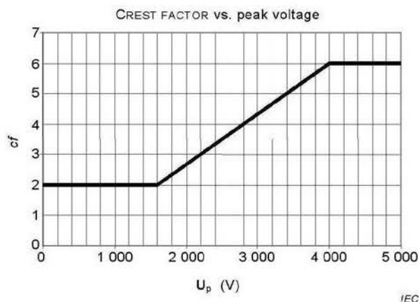
Figure AA.4 – CREST FACTOR vs. peak voltage
