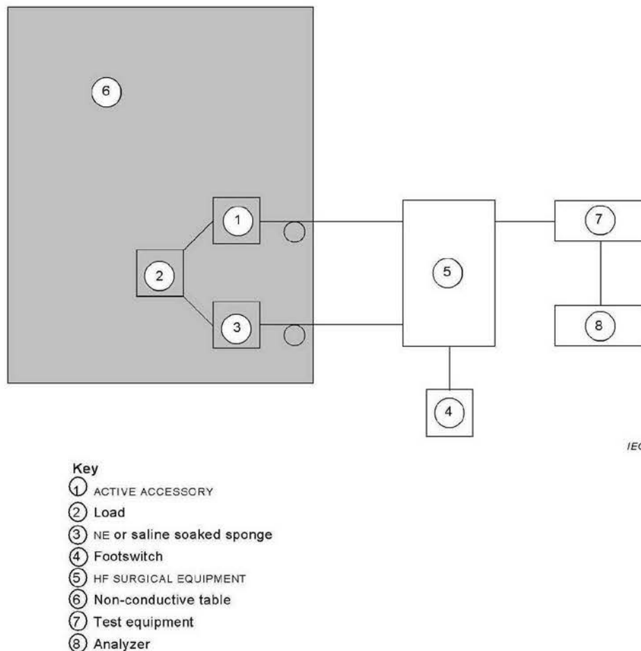
Figure BB.3 – Conducted EMISSIONS test setup
