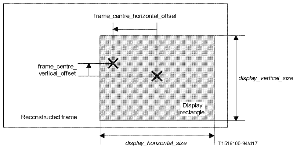
Figure 6-16 – Frame centre offset parameters
