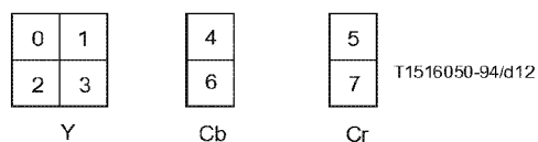
Figure 6-11 – 4:2:2 Macroblock structure
