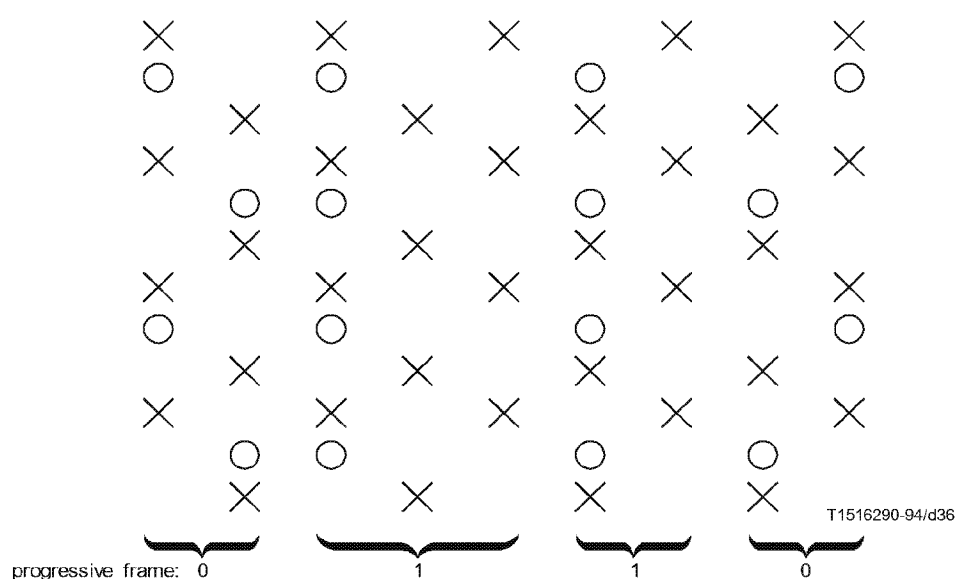
Figure 7-21 – progressive_sequence == 0 with 4:2:0 chrominance
