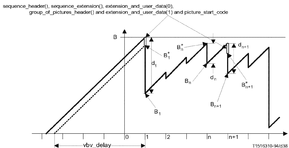
Figure C.1 – VBV Buffer Occupancy – Constant bit-rate operation
