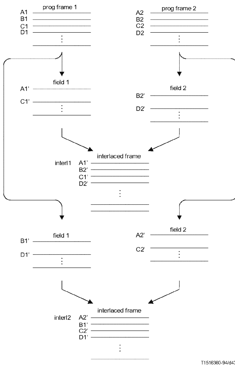
Figure D.3 – Progressive to two interlace conversion
