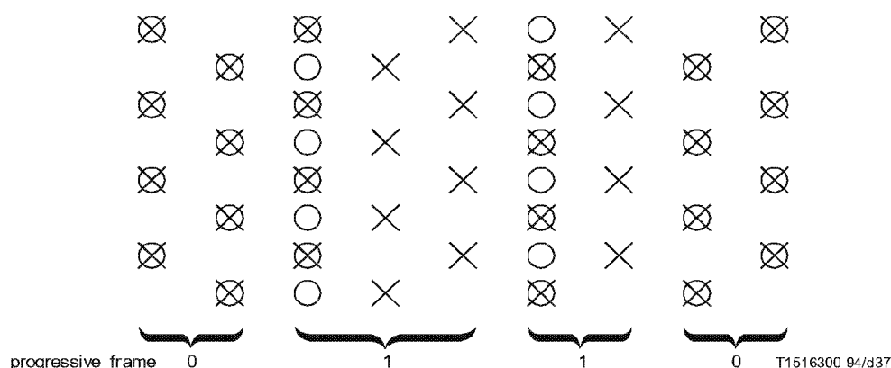
Figure 7-21 – progressive_sequence == 0 with 4:2:0 chrominance
