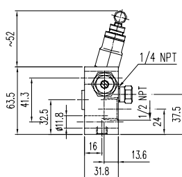
Type 2 (for direct mounting)
