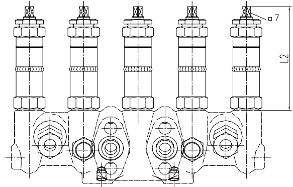
with safety packing (P5 to P6)
