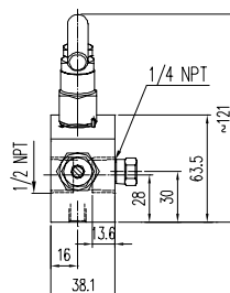
Type 1b (for remote mounting)
