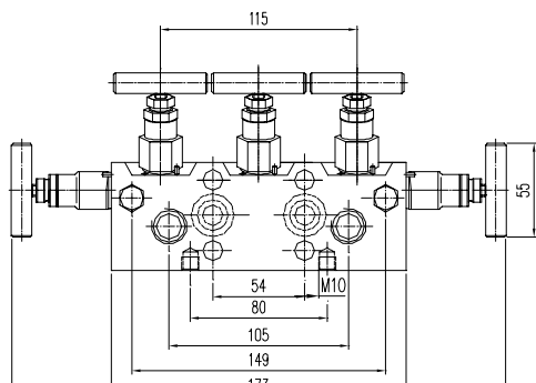
Type 2 (for direct mounting)
