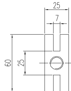
test flange 60 x 25 x 10 mm
