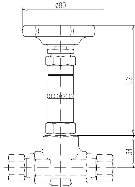
with safety packing (P5 to P6)
