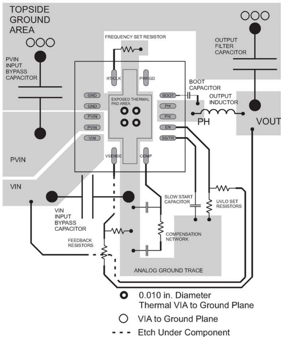
Figure 56. PCB Layout
