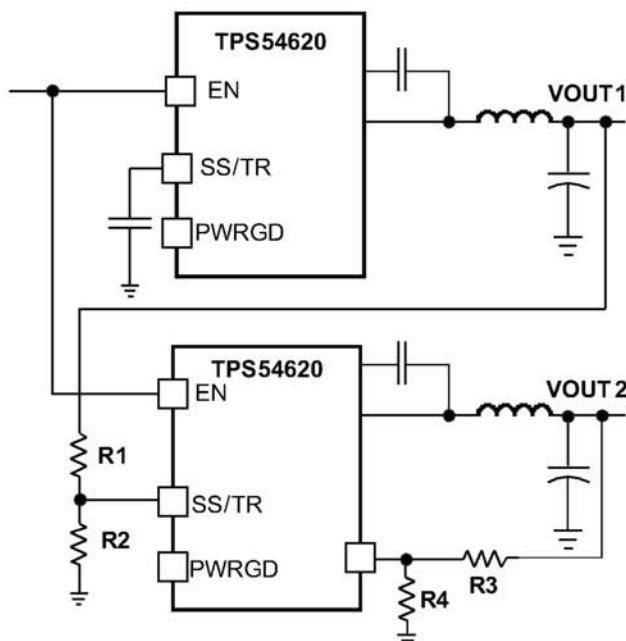
Figure 26. Ratiometric and Simultaneous Startup Sequence
