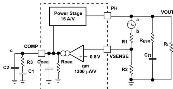
Figure 30. Small Signal Model for Loop Response
