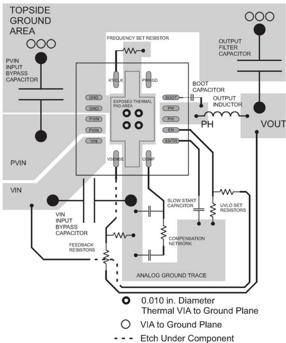
Figure 56. PCB Layout
