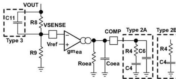
Figure 33. Types of Frequency Compensation
