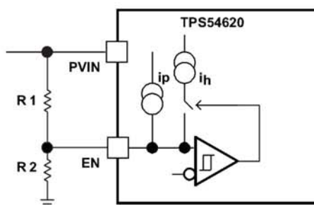
Figure 18. Adjustable PVIN Under Voltage Lock Out, VIN ≥ 4.5V
