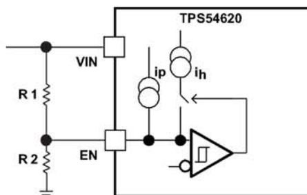
Figure 17. Adjustable VIN Under Voltage Lock Out
