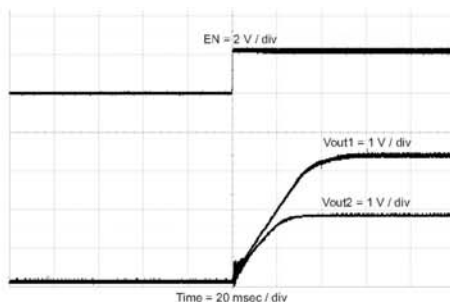
Figure 27. Ratio-metric Startup with Vout1 Leading Vout2
