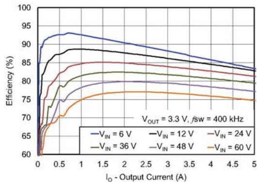
Figure 50. Efficiency vs Load Current
