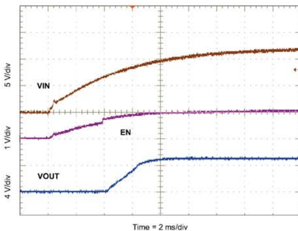
Figure 38. Start-up With VIN
