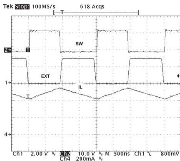
Figure 28. Plot of Synchronizing in CCM
