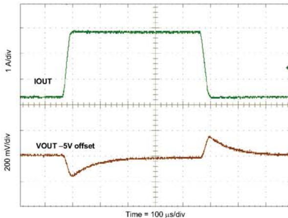
Figure 36. Load Transient
