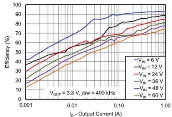
Figure 51. Light Load Efficiency
