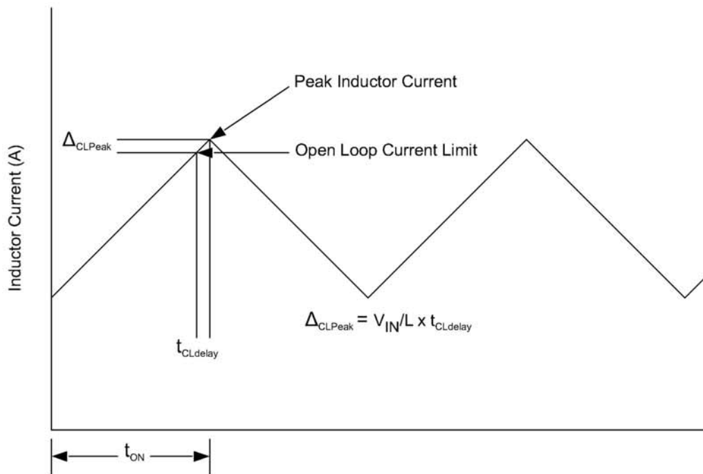
Figure 26. Current Limit Delay
