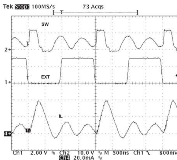
Figure 29. Plot of Synchronizing in DCM
