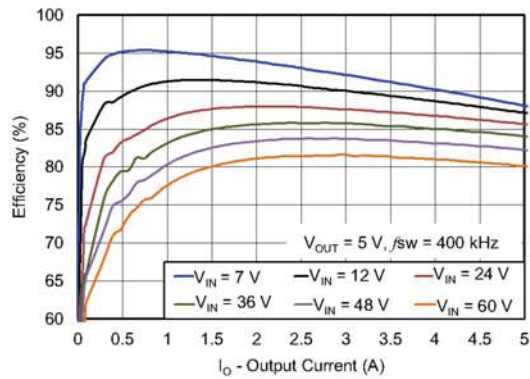
Figure 48. Efficiency vs Load Current
