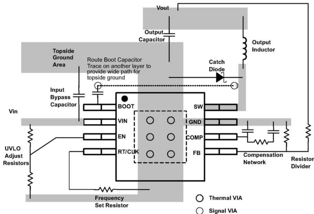
Figure 60. PCB Layout Example
