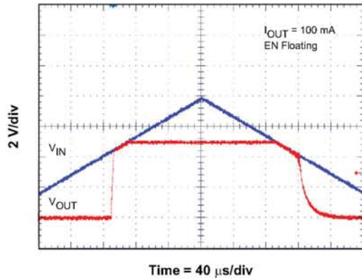
Figure 46. Low Dropout Operation
