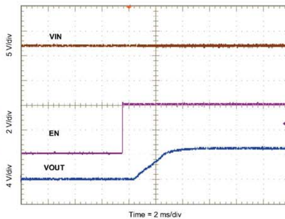
Figure 39. Start-up With EN
