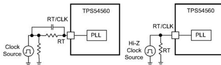
Figure 27. Synchronizing to a System Clock
