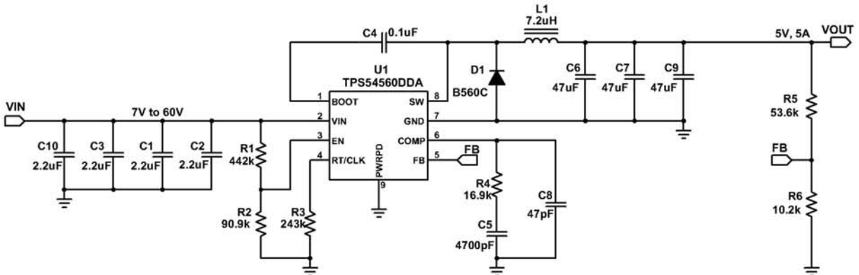
Figure 35. 5 V Output TPS54560 Design Example.
