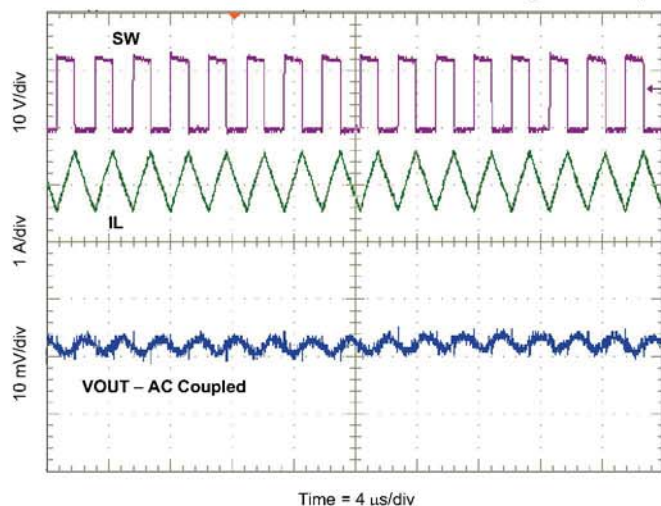
Figure 40. Output Ripple CCM
