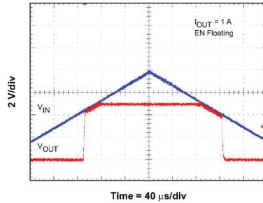
Figure 47. Low Dropout Operation
