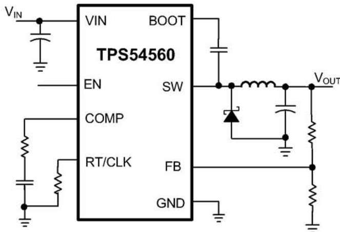
SIMPLIFIED SCHEMATIC
