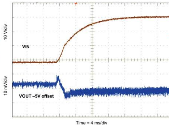
Figure 37. Line Transient (8 V to 40 V)
