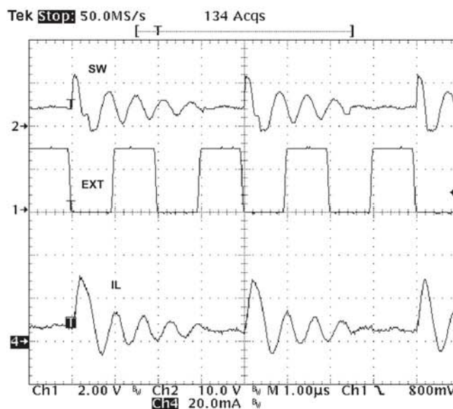
Figure 30. Plot of Synchronizing in Eco-mode
