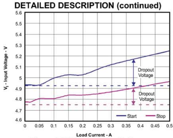
Figure 23. 5V Start/Stop Voltage
