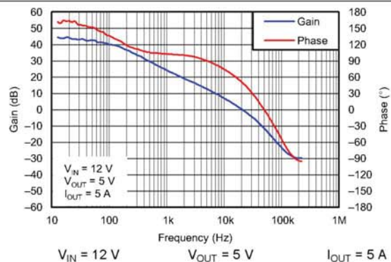
Figure 55. Overall Loop Frequency Response
