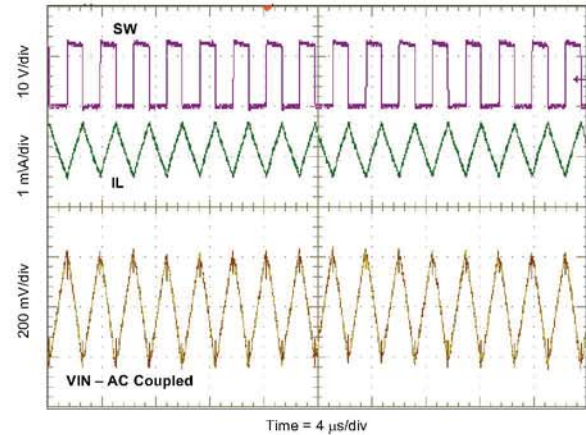
Figure 45. Input Ripple CCM
