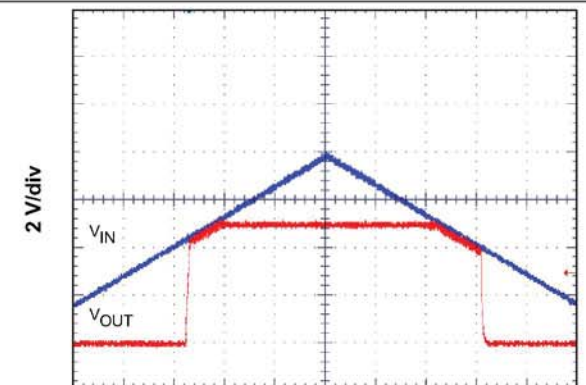
Figure 47. Low Dropout Operation
