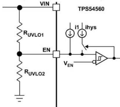
Figure 24. Adjustable Undervoltage Lockout (UVLO)
