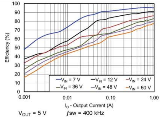
Figure 51. Light Load Efficiency
