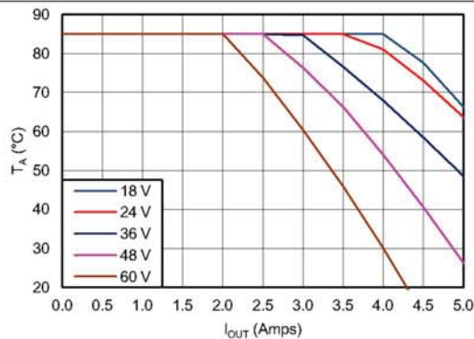
Figure 58. 3.3V Outputs
