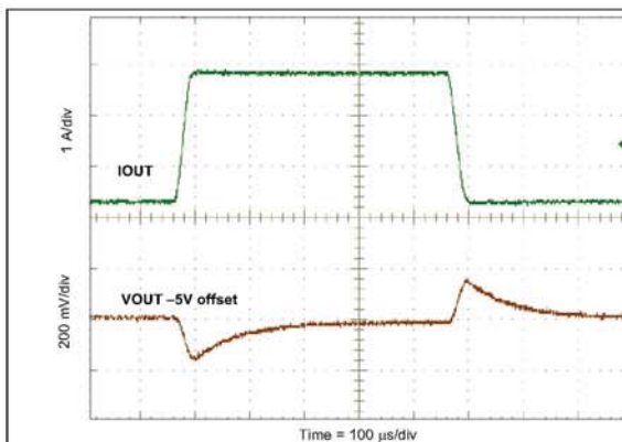
Figure 38. Load Transient
