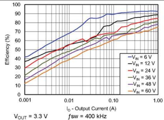
Figure 53. Light Load Efficiency
