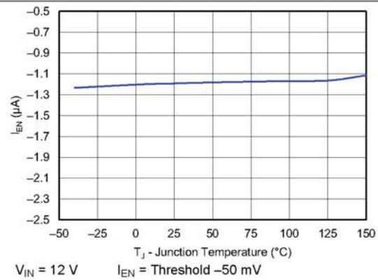
Figure 12. EN Terminal Current vs Junction Temperature
