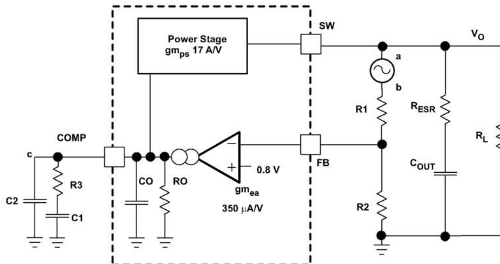
Figure 31. Small Signal Model for Loop Response
