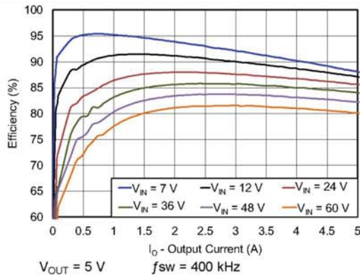
Figure 50. Efficiency vs Load Current
