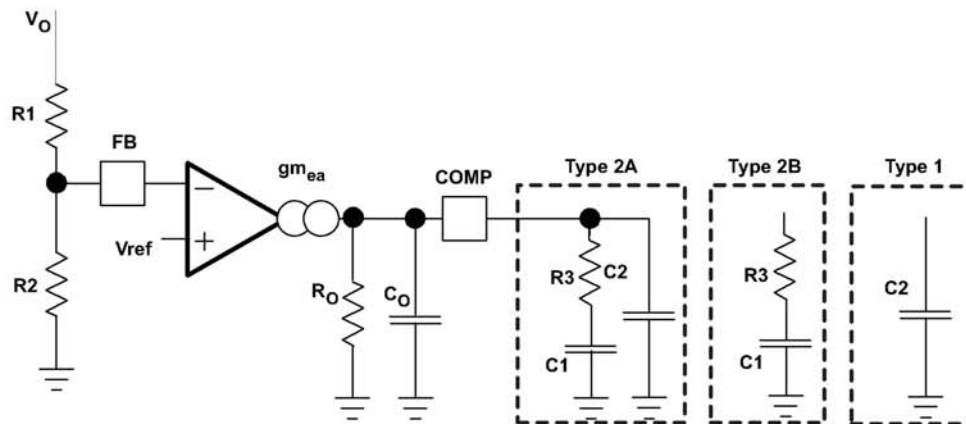
Figure 33. Types of Frequency Compensation
