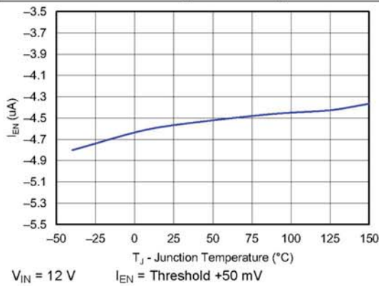
Figure 11. EN Terminal Current vs Junction Temperature
