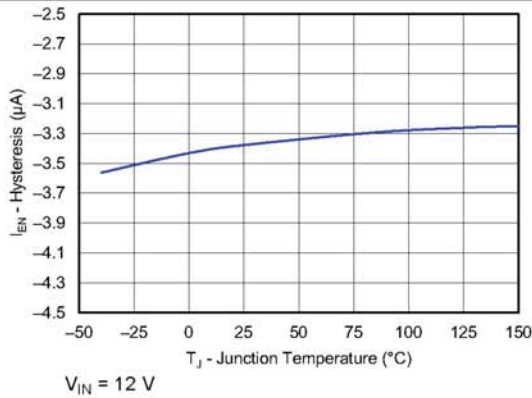
Figure 13. EN Terminal Current Hysteresis vs Junction Temperature
