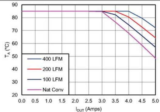
Figure 59. 5V Outputs
