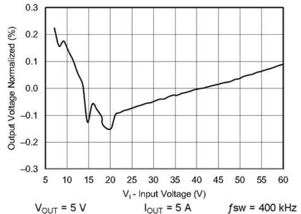
Figure 57. Regulation vs Input Voltage
