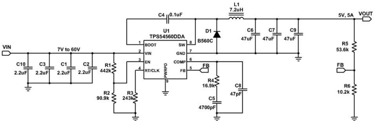
Figure 37. 5 V Output TPS54560 Design Example
