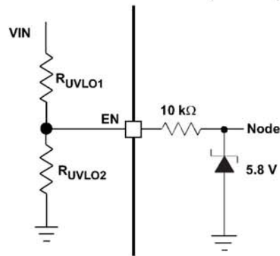
Figure 25. Low Input Voltages Applications
