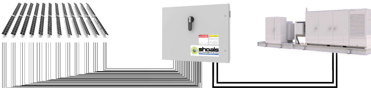
Combiner installation without inline fuse
