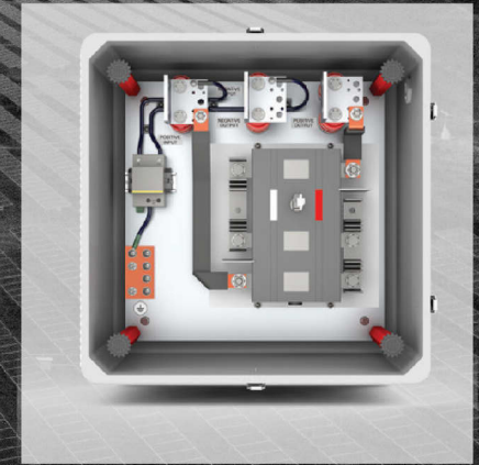
Disconnect Box
