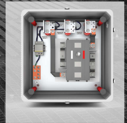
Disconnect Box
