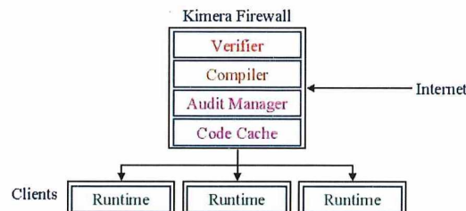
Kimera Firewall Architecture
