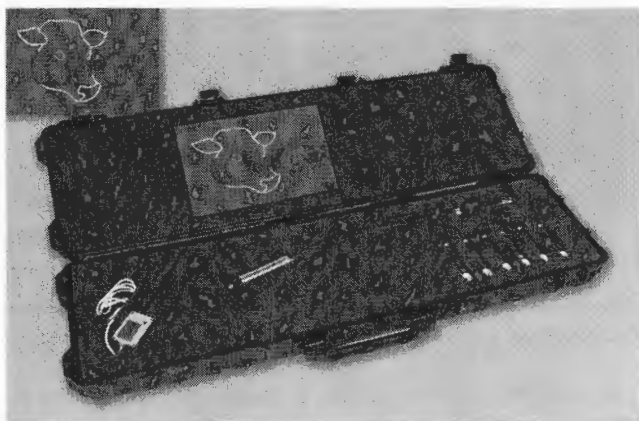
Fig. 3 – Bolus equipment set comprising radio handset for computer attachment, bolting gun and six boluses.
