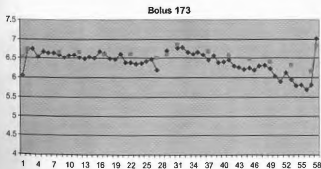
Fig. 4 – Record of bolus and reference pH data over a 14-h period, vertical axis is pH, horizontal axis is the number of automatic samples at 15 min intervals. Squares are manual readings at approximately hourly intervals via fistula, diamonds are the pH telemetry bolus.
