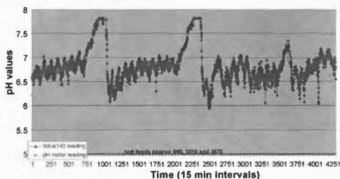
Fig. 5 – Bolus 142 data over a 44-day period compared with reference. The normal daily fluctuation in pH is clear—1–750 = 1 week, followed by a fasting period then a drop following a feed then a return to a normal daily cycle over 10 days then a repeat of the pattern. This graph highlights the different detail of analysis that the novel technology permits.
