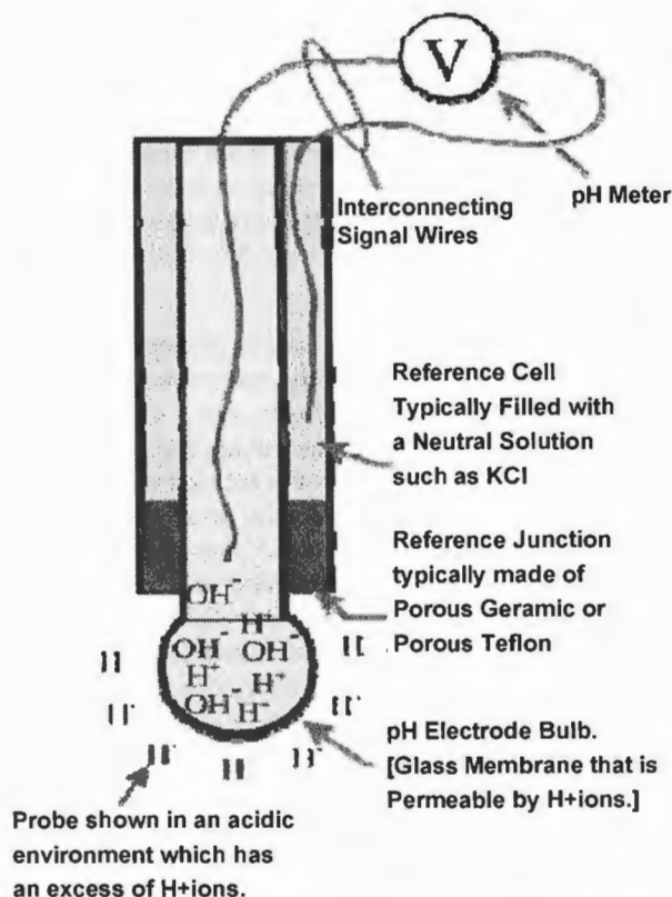
Fig. 1 – Schematic of a laboratory pH sensor, the Well Cow system replaces the pH meter with a microprocessor and radio link to make the device self-contained.
