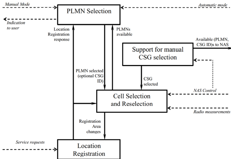
Figure 4.1-1: Overall Idle Mode process
