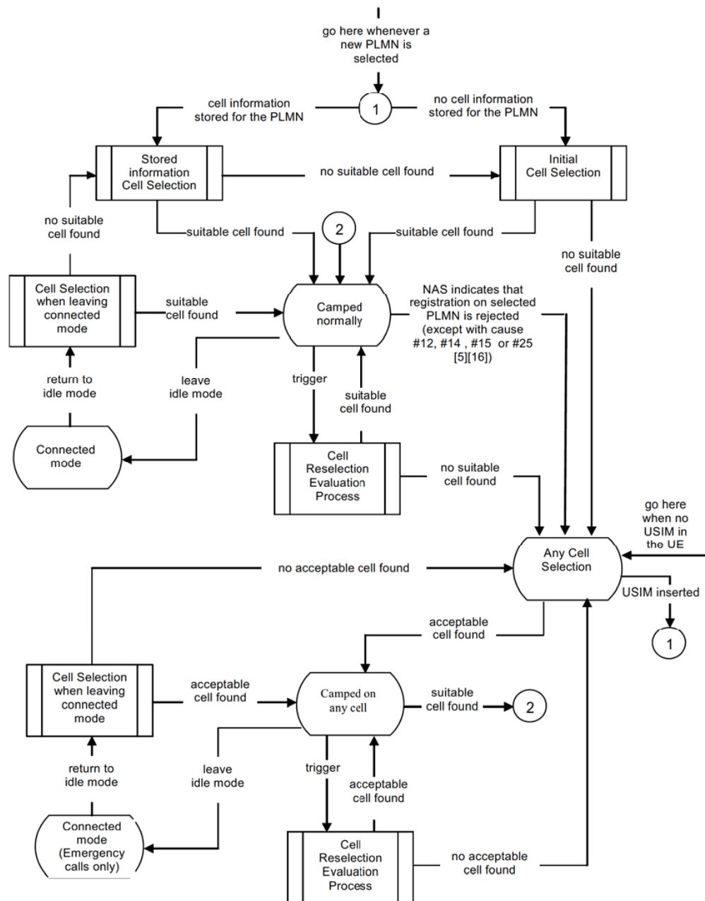
Figure 5.2.2-1: RRC_IDLE Cell Selection and Reselection
