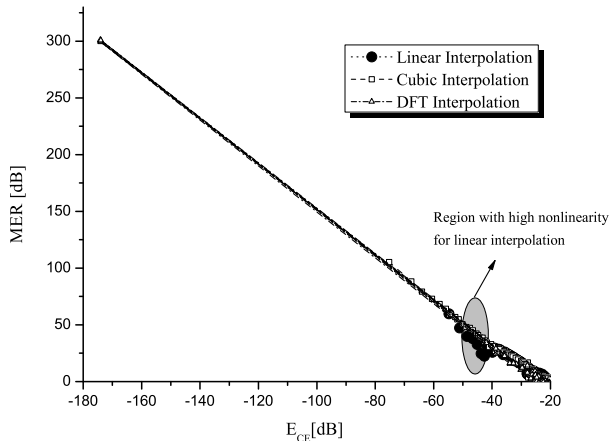
Fig. 17. MER versus E_{CE} both in dB for all interpolation methods analyzed on channel 3.
