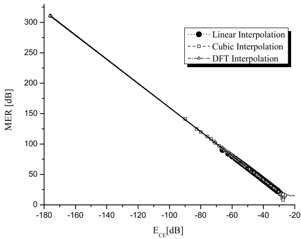
Fig. 16. MER versus E_{CE} both in dB for all interpolation methods analyzed on channel 2.
