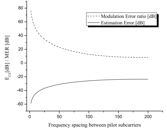
Fig. 13. Channel estimation error and modulation error ratio.
