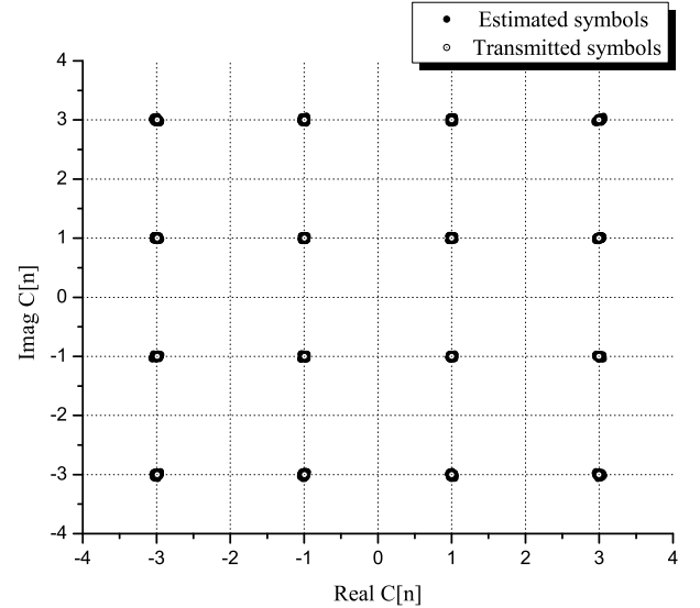
Fig. 9. Symbol dispersion using cubic interpolation.
