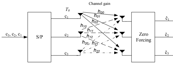
Fig. 3. MIMO system for multiplexing gain.
