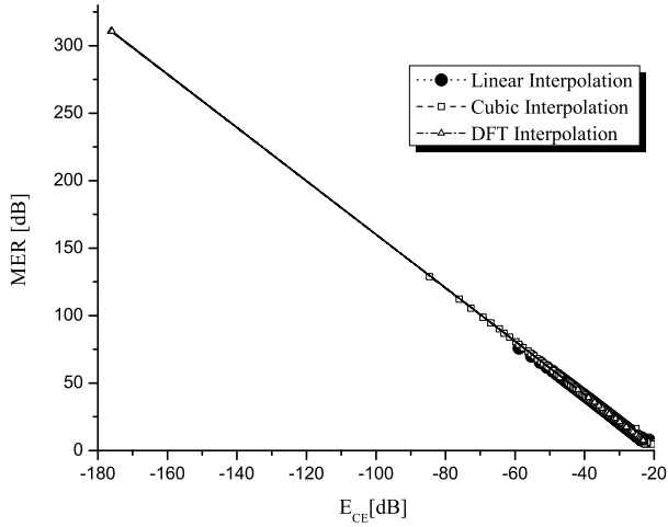
Fig. 15. MER versus E_{CE} both in dB for all interpolation methods analyzed on channel 1.
