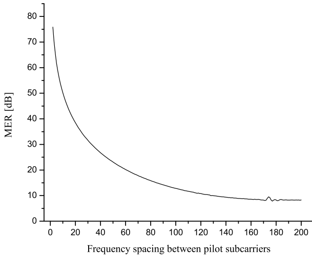
Fig. 12. Modulation error ratio as function of the spacing between pilot subcarriers for linear interpolation.
