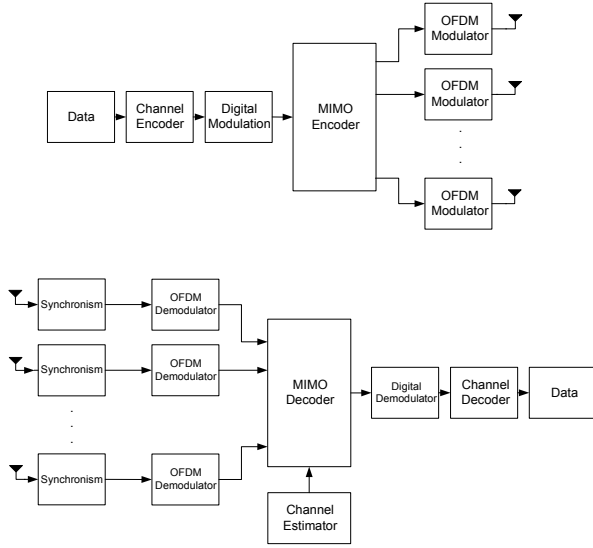
Fig. 6. MIMO-OFDM system.
