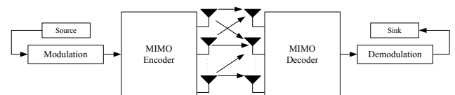
Fig. 1. Basic MIMO system.
