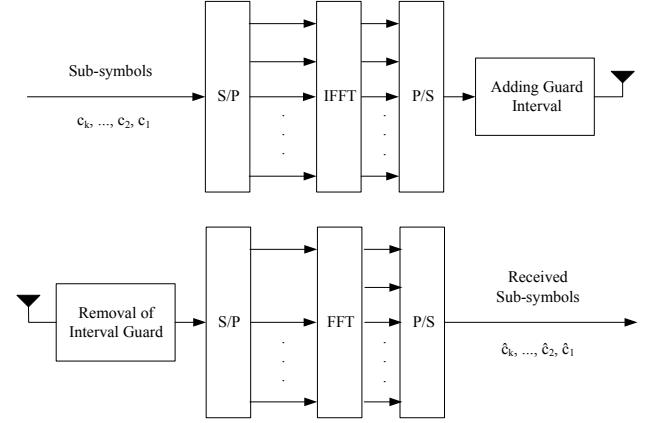
Fig. 5. OFDM system.
