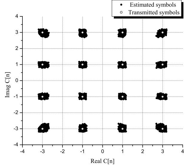
Fig. 8. Symbol dispersion using linear interpolation.
