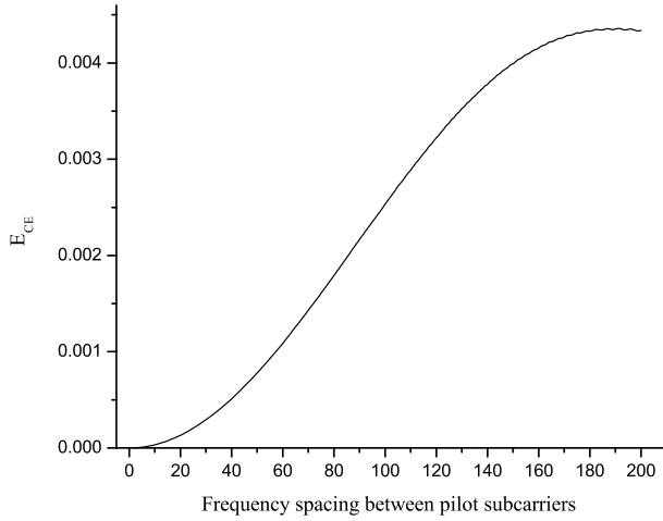
Fig. 11. Channel estimation error as function of the spacing between pilot subcarriers for linear interpolation.
