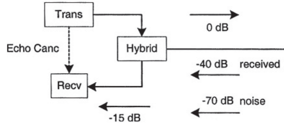
Figure 6.16: An example system illustrating echo cancellation requirement
