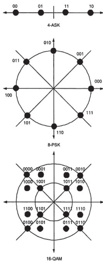
Figure 2.8: Constellation diagram
