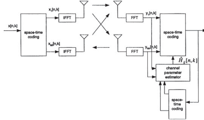
Figure 6.9: MIMO-OFDM architecture
