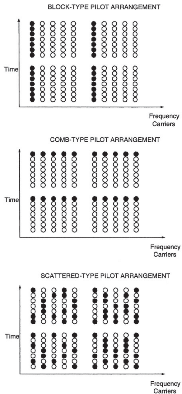
Figure 6.4: Pilot arrangement
