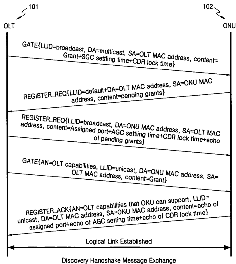
FIG. 5 (PRIOR ART)
