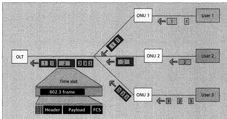
■ Figure 5. Upstream traffic in EPON.
