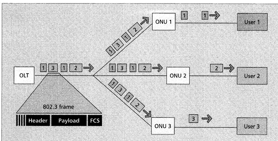
■ Figure 4. Downstream traffic in EPON.
