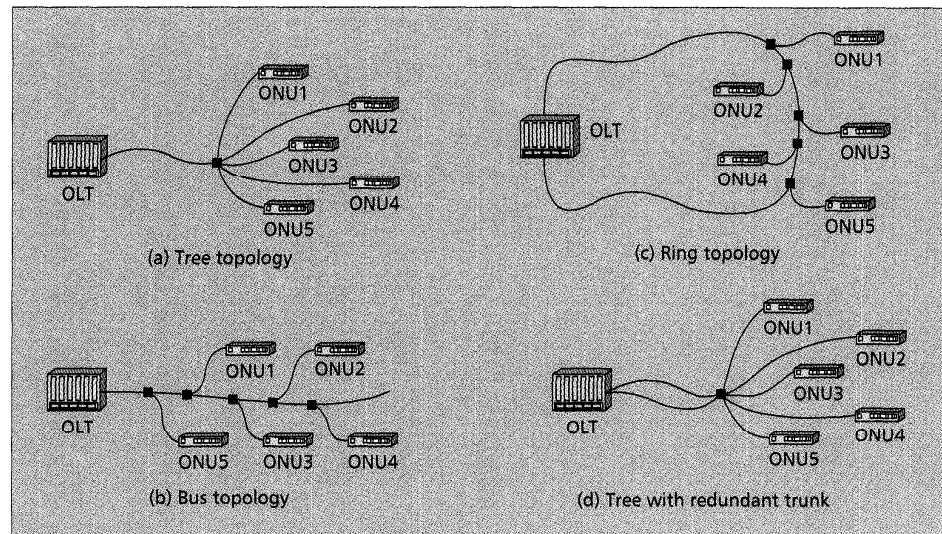
■ Figure 3. PON topologies.
