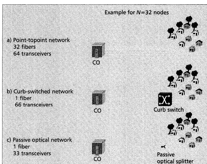
Figure 2. Fiber to the home (FTTH) deployment scenarios.
