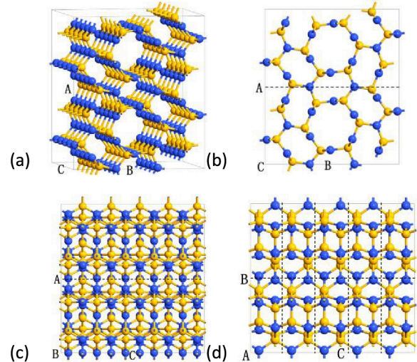
Figure 3. (a), (b) The supercell structure and (c), (d) their side views, including 280 atoms (expand the unit cell with 2 \times 1 \times 5 at the A, B, and C direction respectively, A = 12.9879 Å, B = 14.9971 Å, and C = 14.3566 Å).
