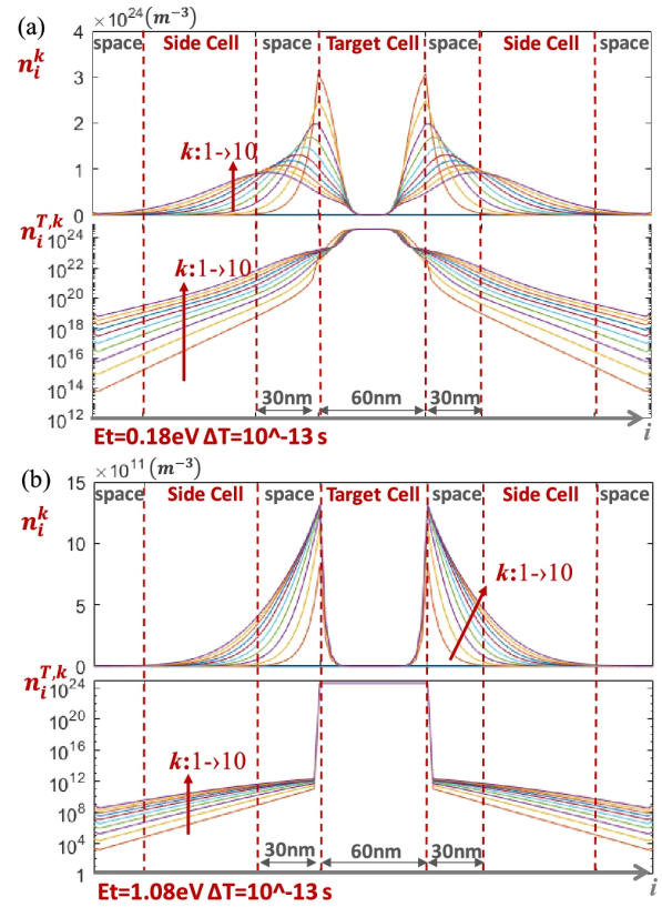
Figure 10. Distribution of electrons in the conduction band (up) and the traps (down) with (a) V_{\text{N-O}_i} with 0.18 eV trap level and (b) V_{\text{N-OH}_i} with 1.08 eV trap level.
