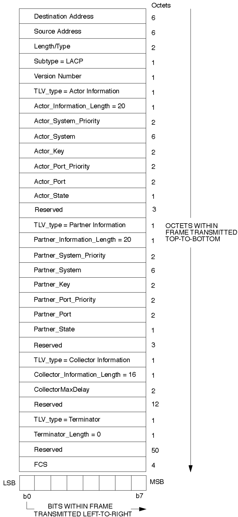
Figure 43-7 – LACPDU structure
