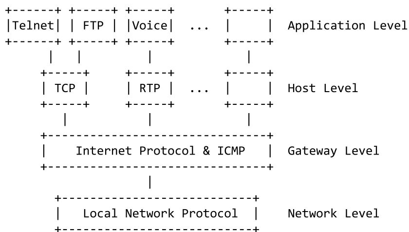
Protocol Relationships
