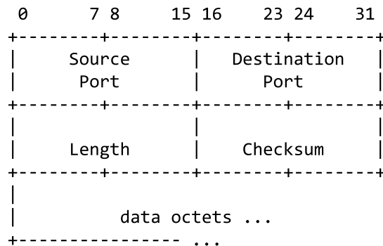
User Datagram Header Format
