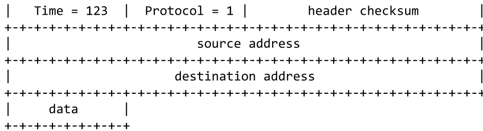
Example Internet Datagram
