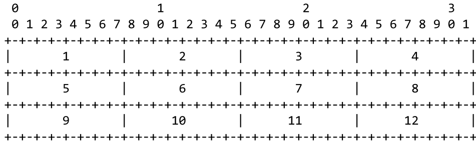
Transmission Order of Bytes
