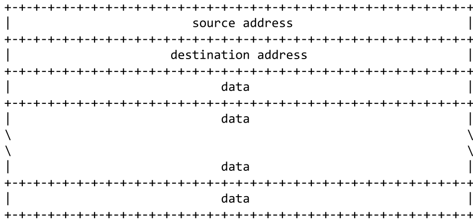
Example Internet Fragment
