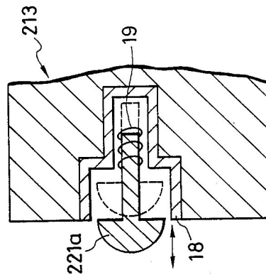
FIG. 3 PRIOR ART
