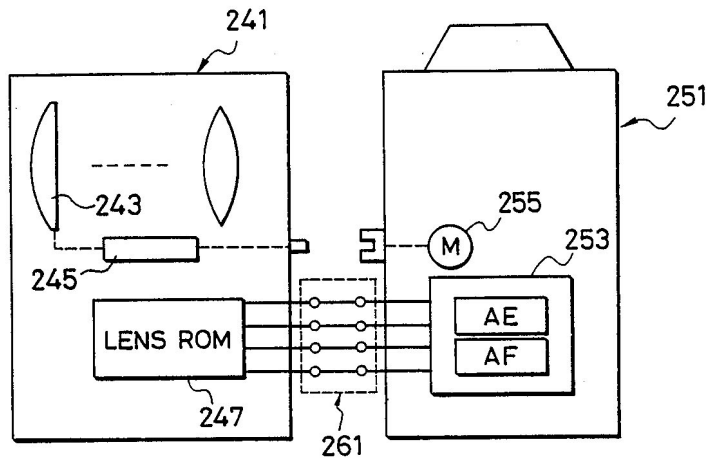
FIG. 5 PRIOR ART
