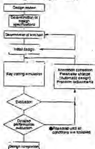
Figure-1 Lens Design Process Flow (general design procedure)
