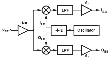
Fig. 1. Receiver architecture.
