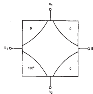
4-Port Hybrid with Phase and Isolation
