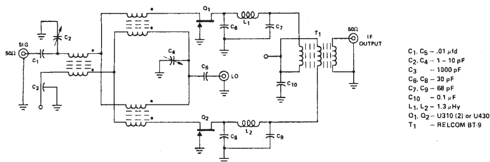
Prototype Active Balanced Mixer
