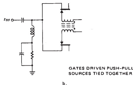
Alternate Forms of L.O. Injection
