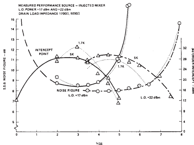
Noise Figure and Intercept Point Performance
