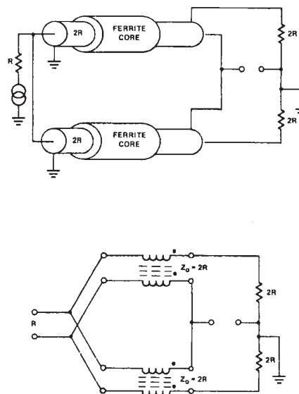
Hybrid Input Coupling Transformer
