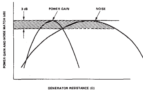
Power Gain and Noise Matching Figure 6
