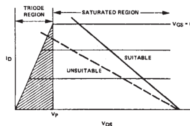
Plotting Drain Load Lines Figure 4
