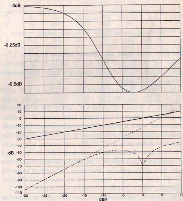
Fig. 8. Harmonic signature for the 50- \Omega -padded MICROMIXER ( I_Z = 517 \mu\text{A} ). Top panel: gain error of fundamental; bottom panel: fundamental, actual HD3, and extrapolation.
