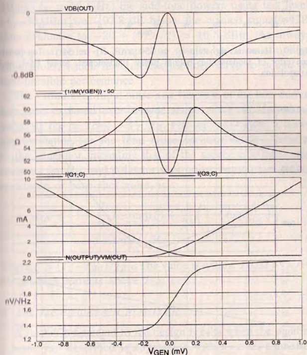
Fig. 7. Swept- V_{\text{GEN}} results for 50- \Omega -padded MICROMIXER ( I_2 = 517 \mu\text{A} ). Compare with Fig. 4.
