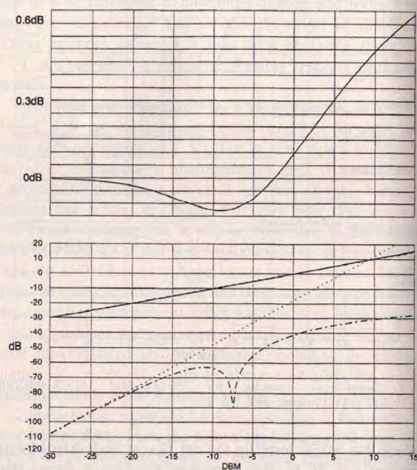
Fig. 11. Harmonic signature I_Z = 430 \mu AP, R_P = 40 \Omega . Top panel: gain error of fundamental; bottom panel: fundamental, actual HD3, and extrapolation.
