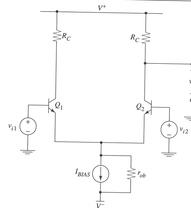
► Figure 11.20 Differential amplifier with single-ended output.
