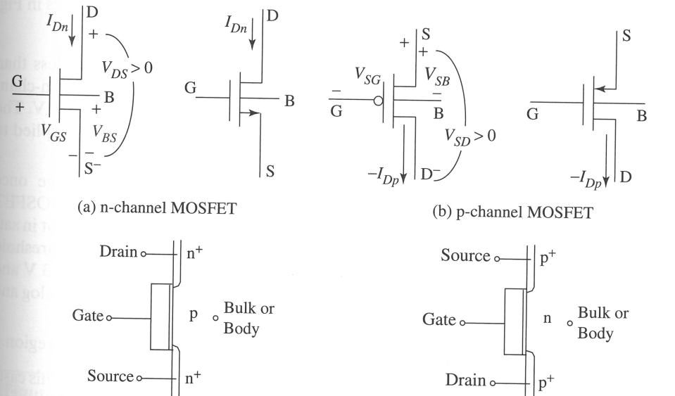
► Figure 4.2 (a) n-channel MOSFET symbols and structure and (b) p-channel symbols and structure.
