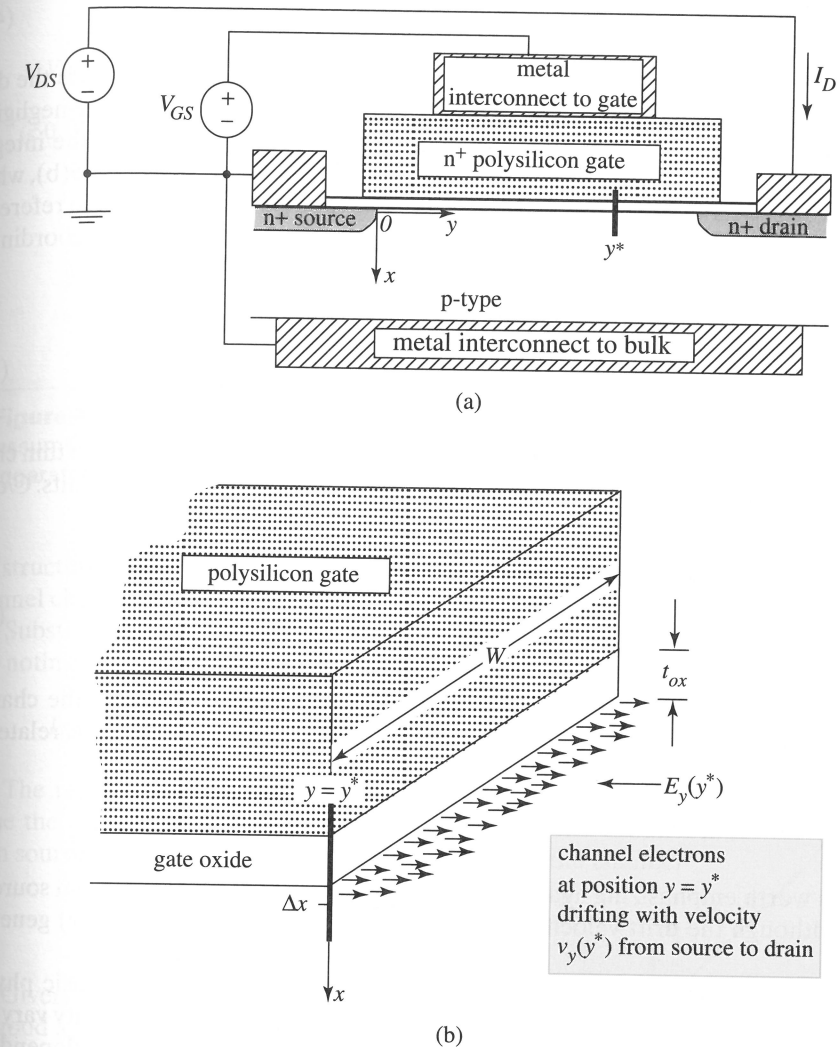
► Figure 4.5 (a) MOSFET biased with V_{GS} > V_{TN} and V_{DS} > 0 . (b) Cutaway view of drifting electrons in the channel at position y^* (see (a)) between the source ( y = 0 ) and drain ( y = L ).
