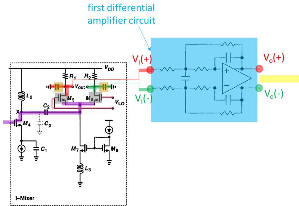
Combined Receiver (using circuit of TI-1021/1022)
