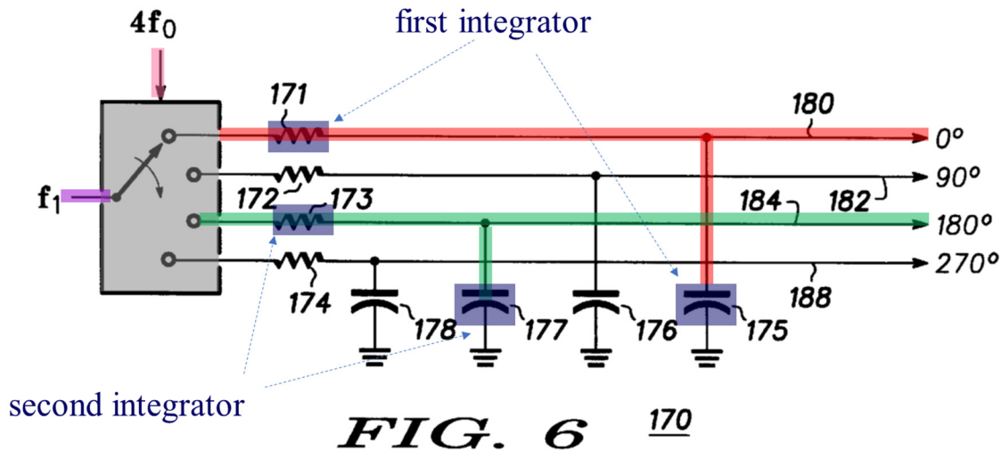
TI-1004, Figure 6 (annotated)
