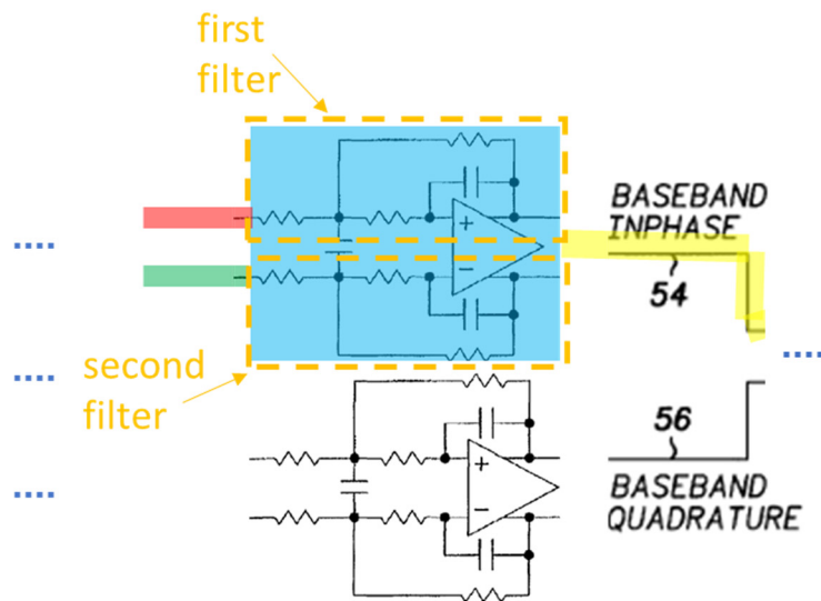
Combined System (zoomed portion using circuits of TI-1021/TI-1022)
