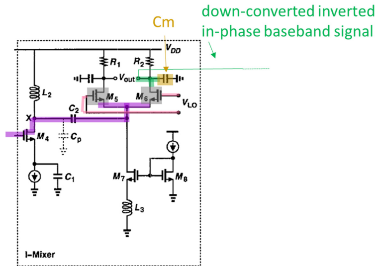
TI-1017, Fig. 2 (annotated)
