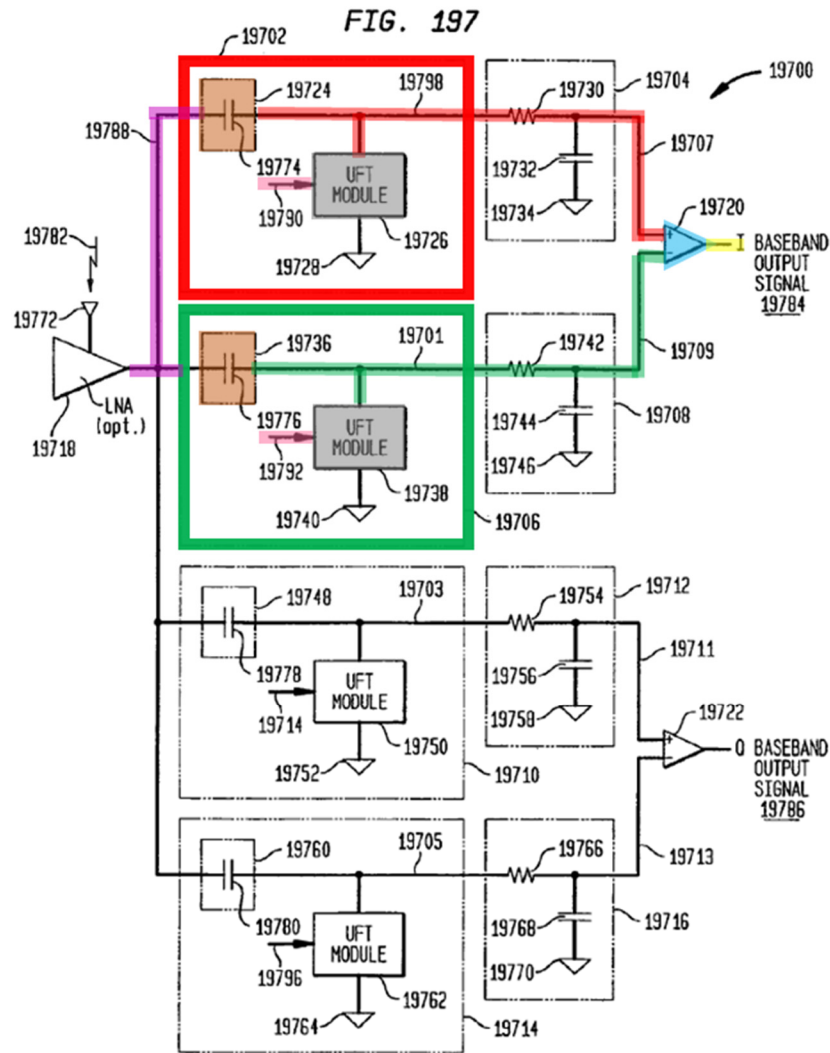
TI-1001, FIG. 197 (annotated)
