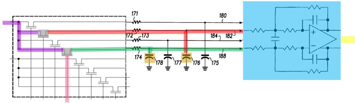
Combination System (using switch of TI-1005 and circuit of TI-1021)
