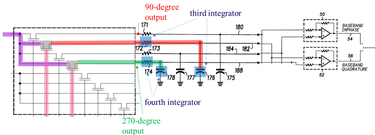
Combination System (using switch of TI-1005)
