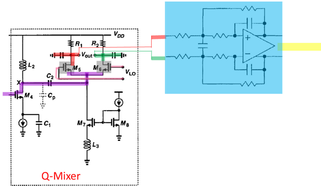
Combination Receiver (using circuits of TI-1021/TI-1022)
