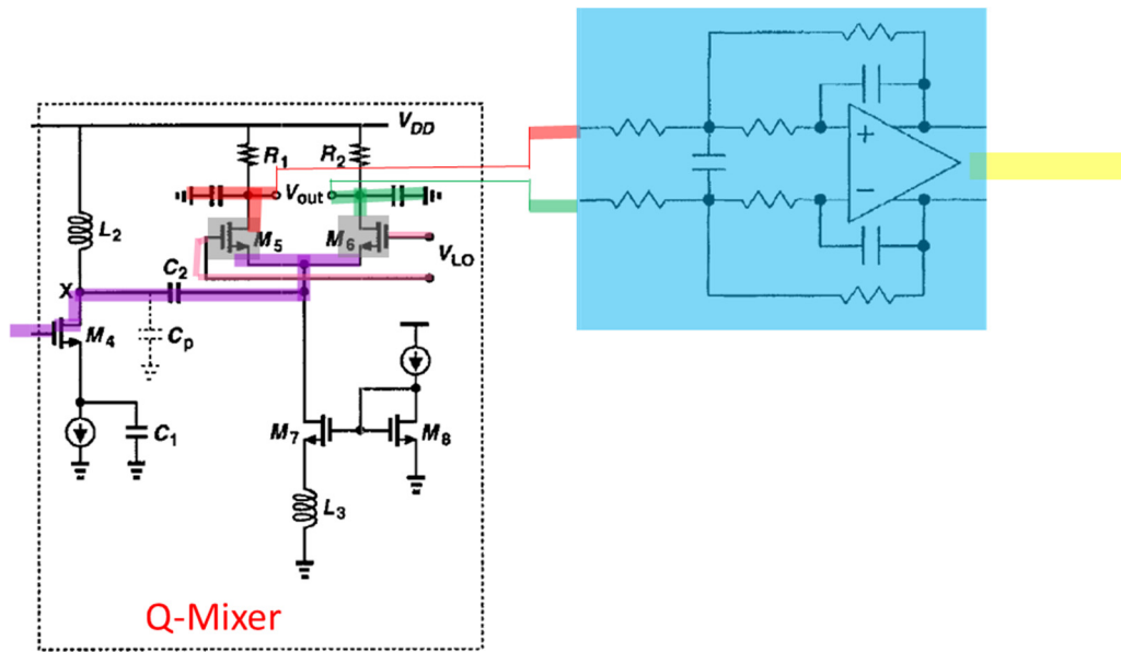
Combination Receiver (using circuit (light blue) of TI-1021/TI-1022)
