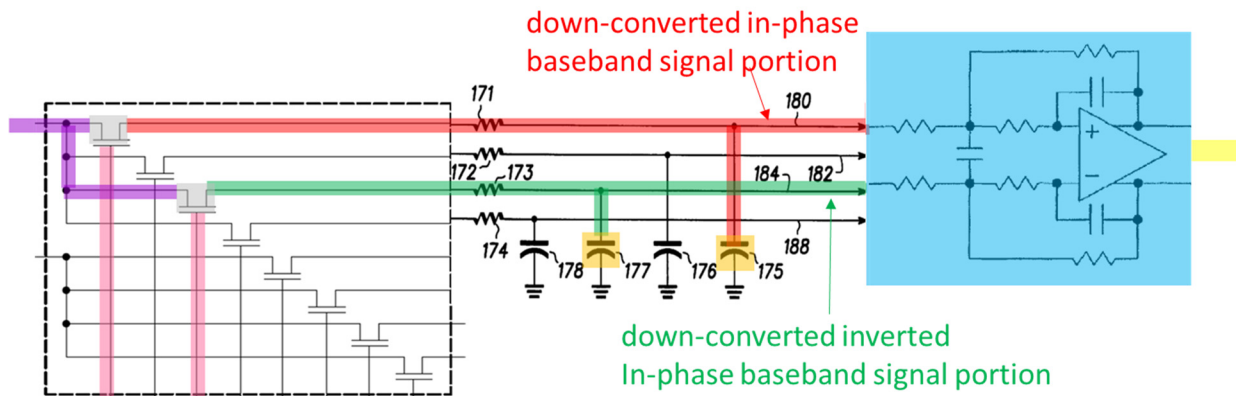
Combination System (using switch of TI-1005 and circuit of TI-1021/TI-1022)
