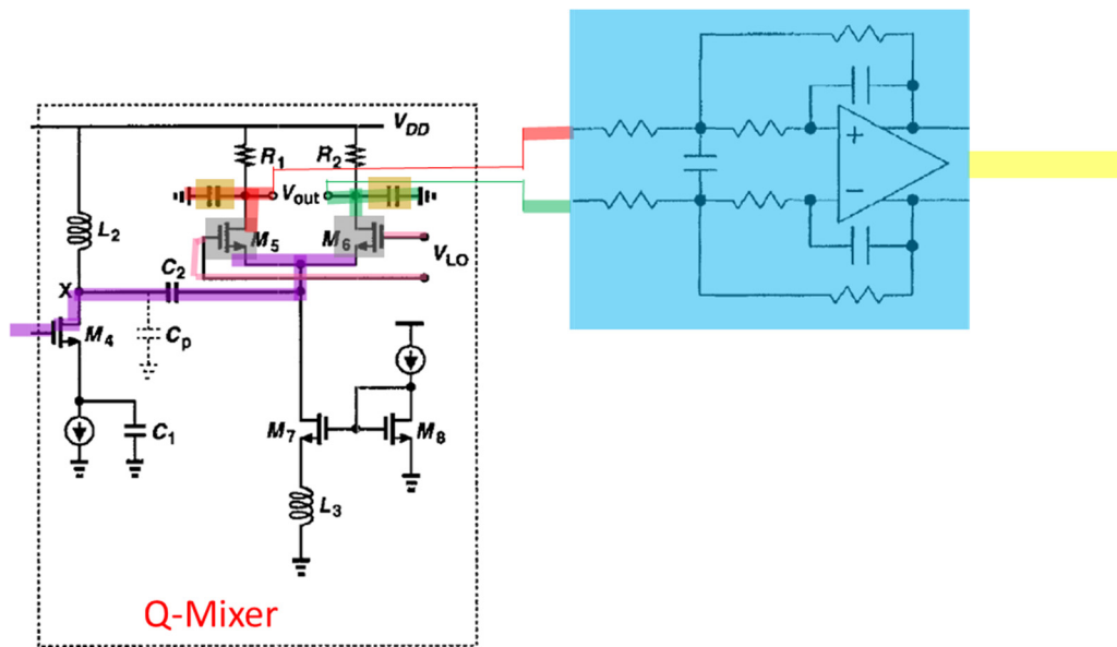
Combination Receiver (using circuits of Macnally)
