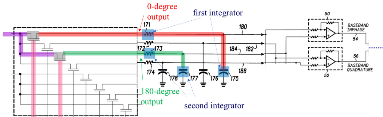
Combination System (using switch of TI-1005)
