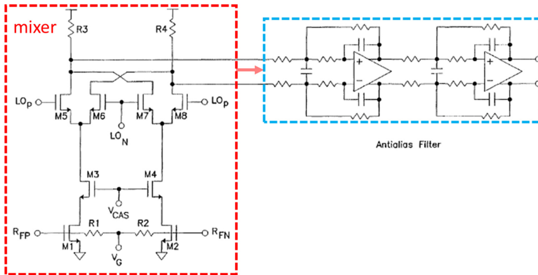
TI-1021/TI-1022, Fig. 3 (annotated)
