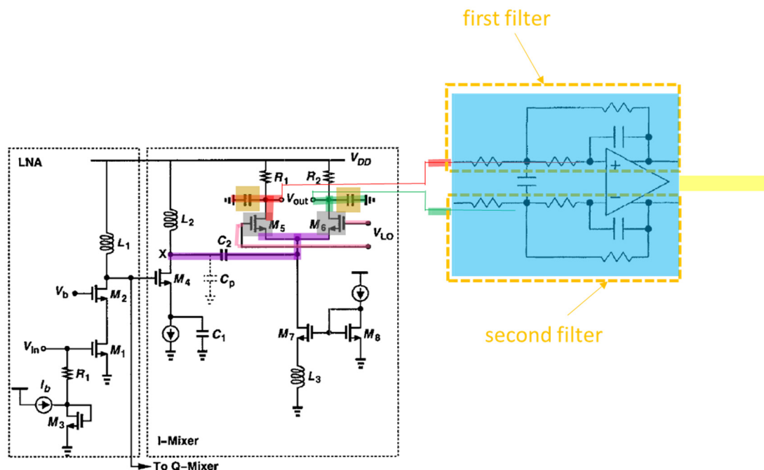
Combined Receiver (using circuit of TI-1021/TI-1022)
