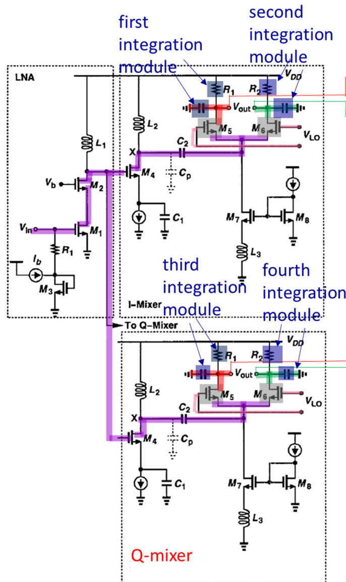
Combination Receiver (zoomed portions of I-mixer/Q-mixer of TI-1017)
