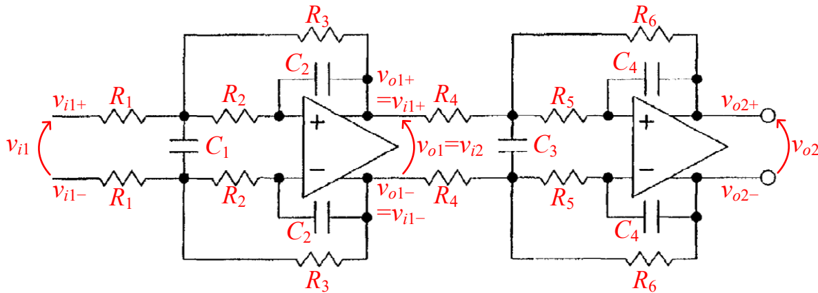
Figure 1: Annotated copy of the antialiasing filter shown in Fig. 3 of Macnally(TI-1021/TI-1022)
