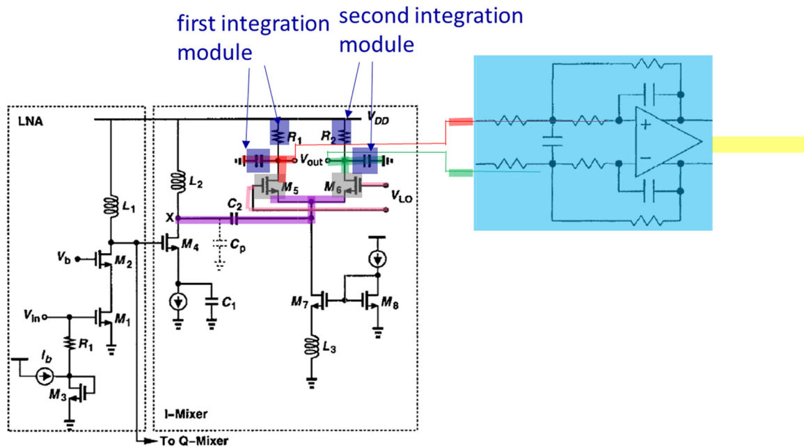
Combined Receiver (using Macnally's circuit for baseband processing)
