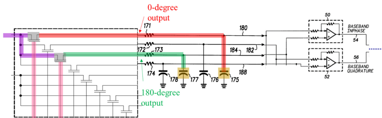
Combination System (using switch of TI-1005)
