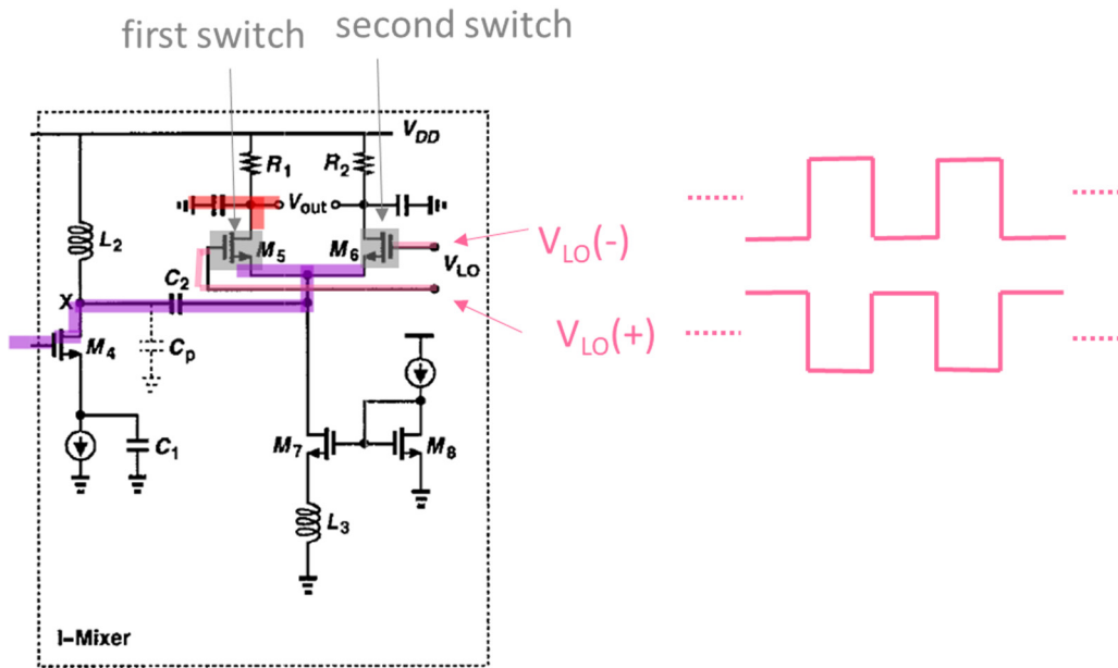
TI-1017, Fig. 2 (annotated)
