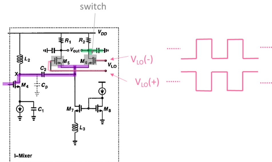
TI-1017, Fig. 2 (annotated)
