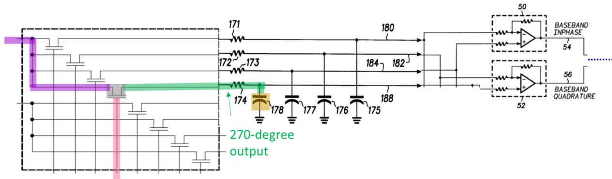
Combination System (using switch of TI-1005)
