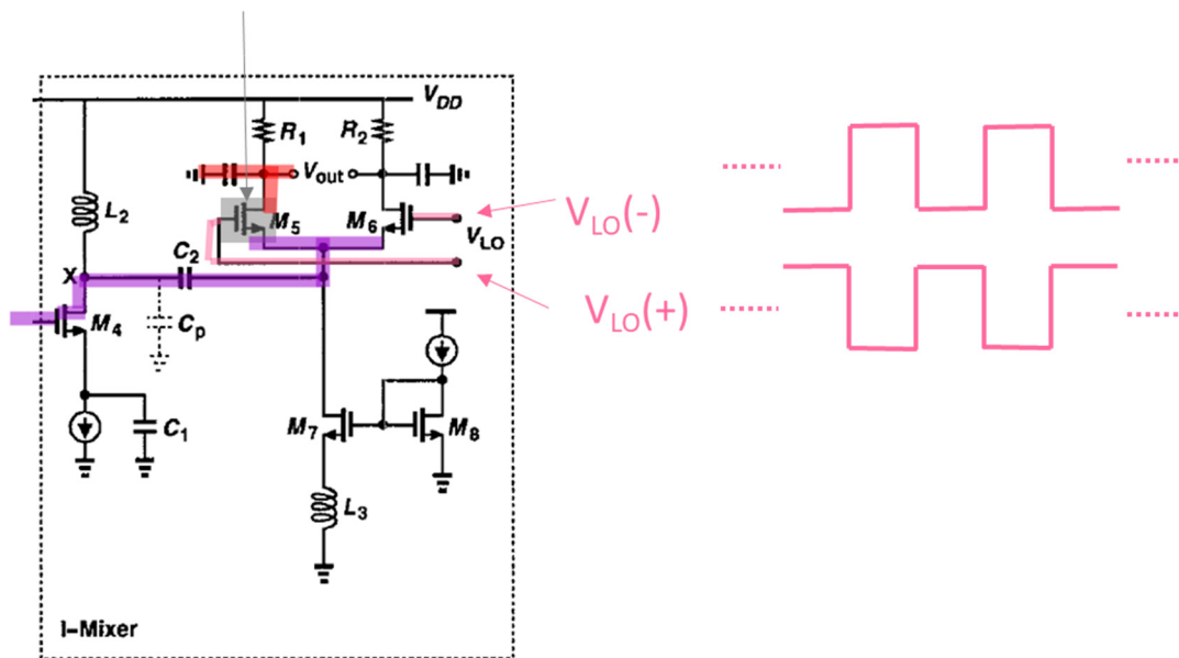
TI-1017, Fig. 2 (annotated)
