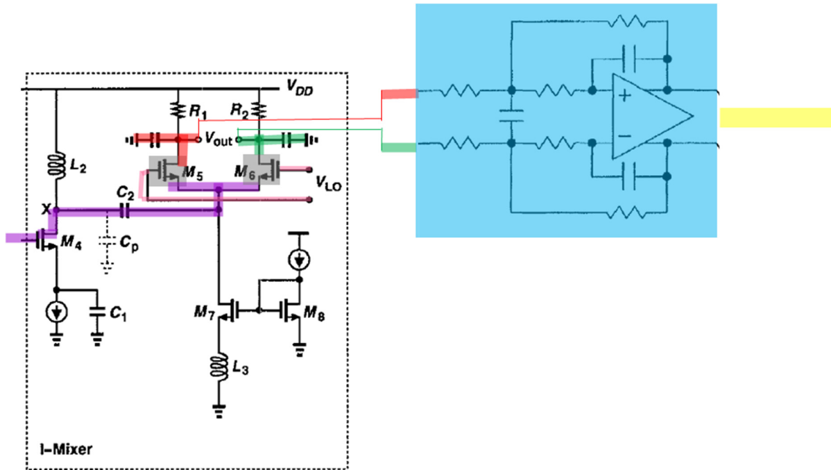
Combination Receiver (using Macnally's circuit (light blue))
