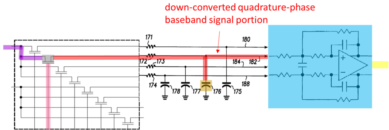
Combination System (using switch of TI-1005 and circuit of TI-1021)
