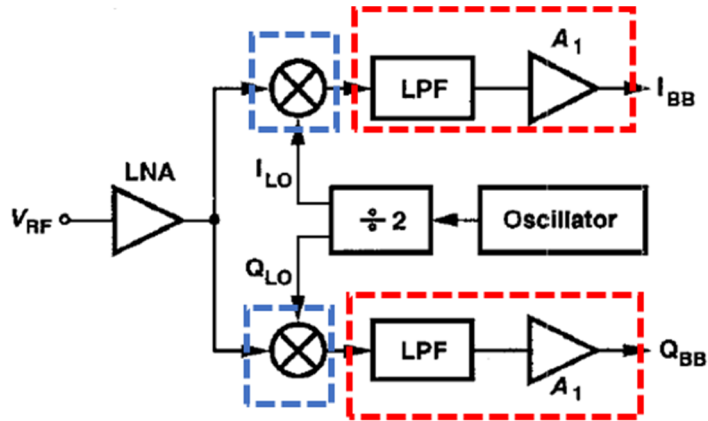
Fig. 1. Receiver architecture.
