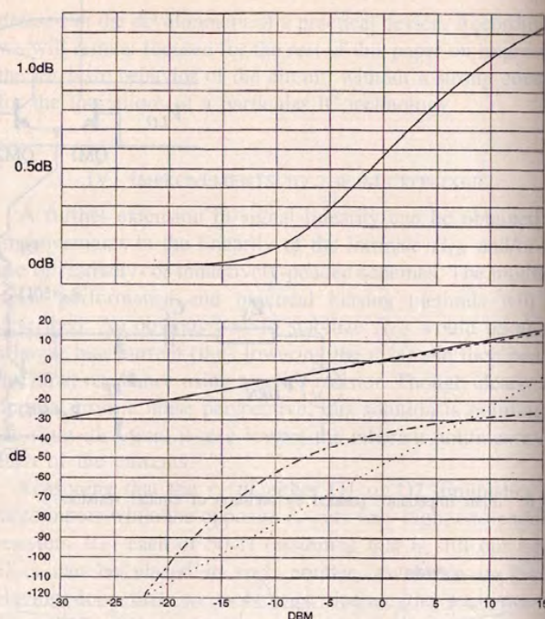
Fig. 10. Harmonic signature I_Z = 390 \mu\text{AP} , R_P = 34 \Omega . Top panel: gain error of fundamental; bottom panel: fundamental, actual HD3, and extrapolation.
