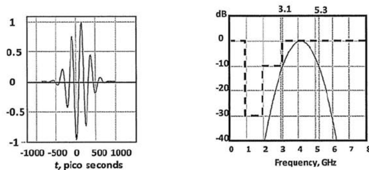
Fig. 1: UWB waveform shown in time domain (at left) and frequency domain (at right)
