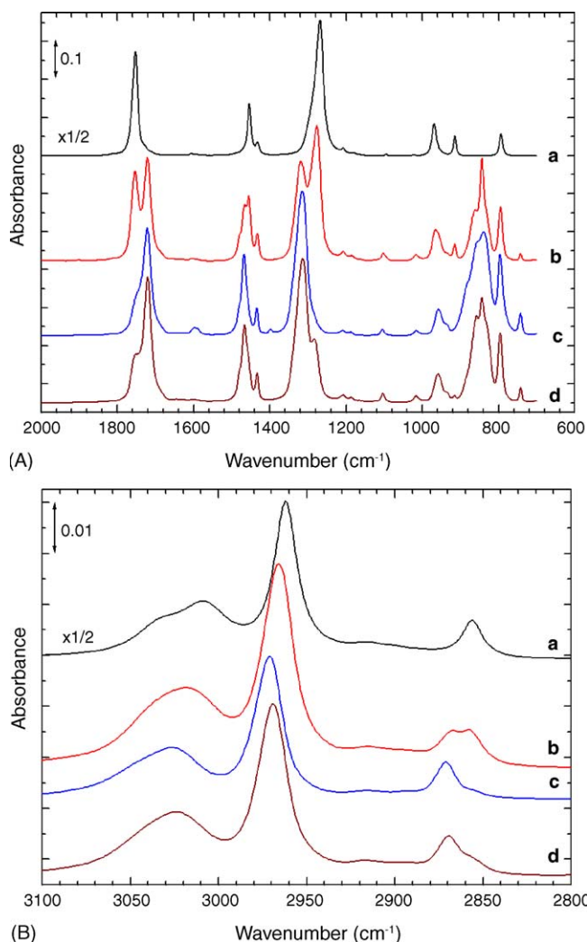
Fig. 7. Same experiment as in Fig. 6 for 1 m LiPF 6 /DMC: (a) pure DMC; (b) 1 m LiPF 6 /DMC solution; (c) after storage at 85 °C for 300 h; and (d) with 300 ppm H 2 O added.
