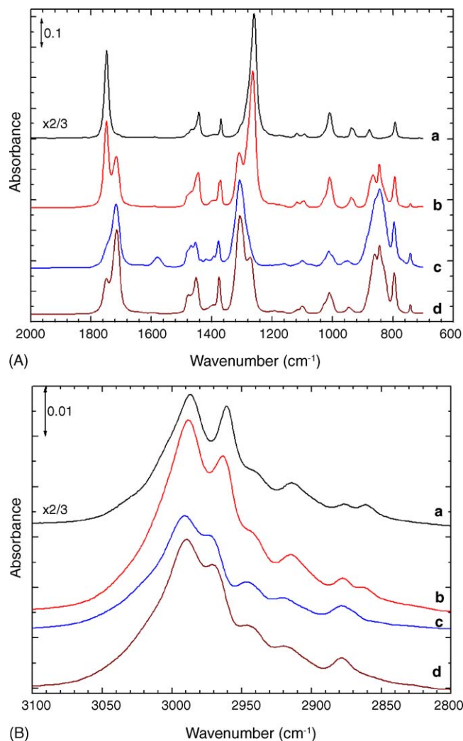
Fig. 8. Same experiment as in Fig. 6 for 1 m LiPF 6 /EMC solution: (a) pure EMC; (b) 1 m LiPF 6 /EMC solution; (c) after storage in closed container under vacuum at 85 °C for 300 h; and (d) with 300 ppm H 2 O added.
