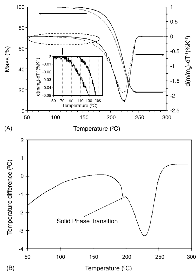
Fig. 1. (A) Mass loss (left) and rate of mass loss (right) during thermal decomposition of LiPF 6 at a heating rate of 10 °C min −1 in argon (flow rate: 220 ml min −1 ) containing <10 ppm H 2 O (solid line) and with 300 ppm water vapor (dashed line); (B) derivative thermal analysis (DTA) profile in the same experiment.
