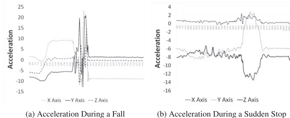
Fig. 7. Acceleration During Falls and Sudden Stops
