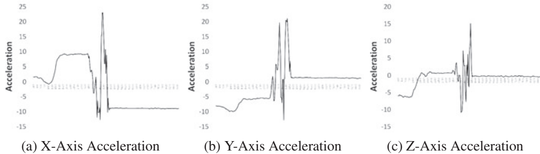
Fig. 8. Acceleration During a Sudden Stop
