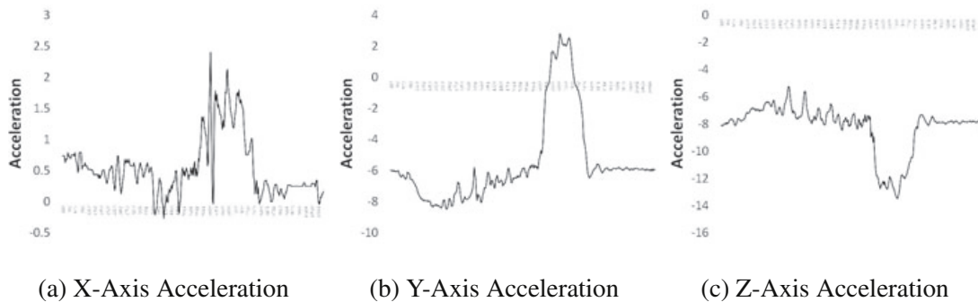
Fig. 9. Acceleration While Dropped in a Car
