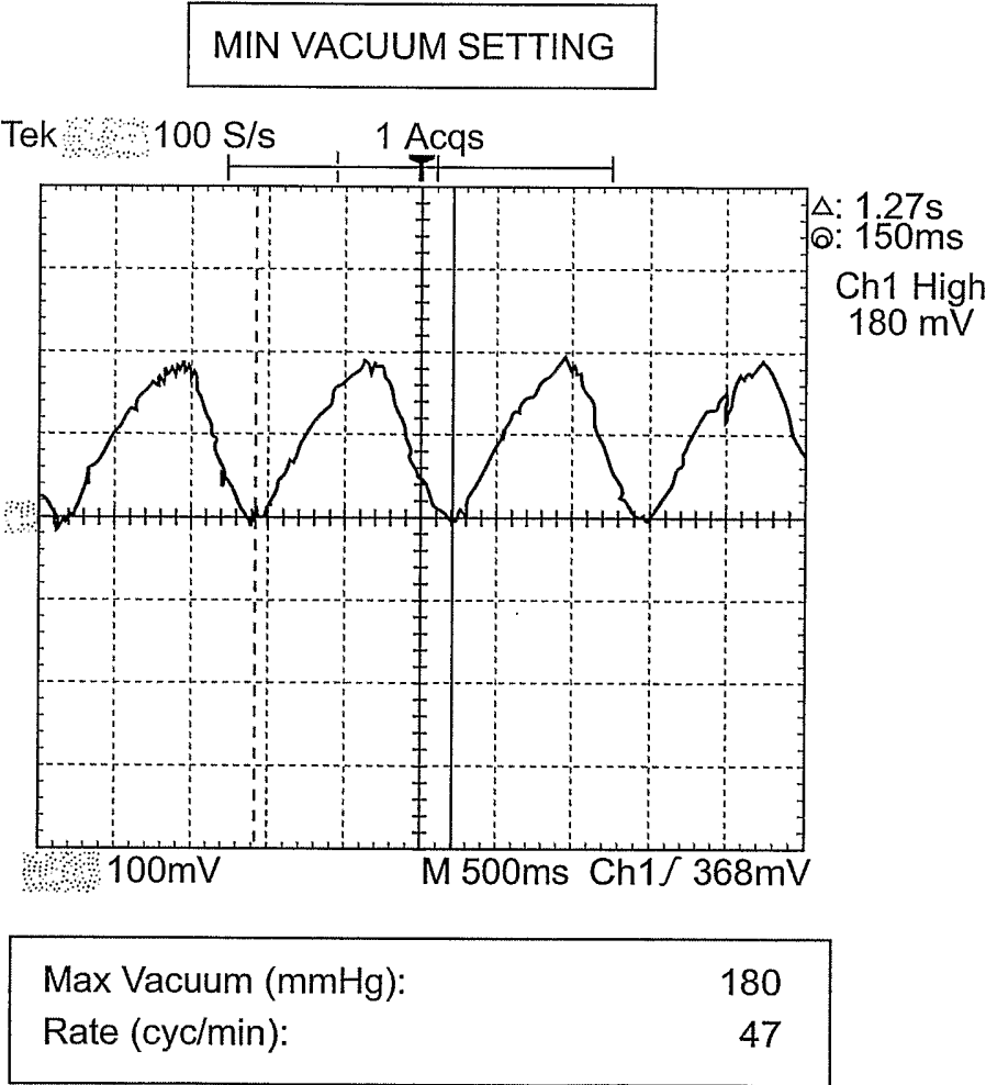
FIG. 24B PRIOR ART
