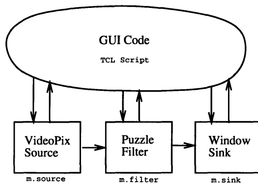
Figure 4.3: A block diagram of the puzzle application.
