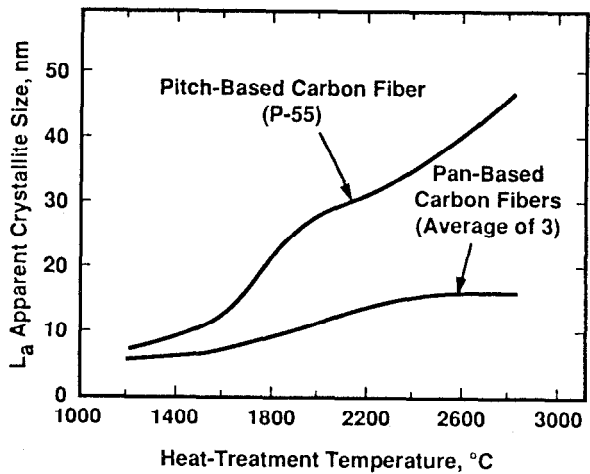
Figure 8.7. Apparent crystalline size ( L_a ) of PAN-based and pitch-based carbon fibers as a function of heat-treatment temperature. [7]
