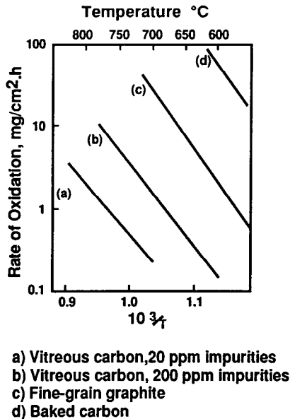
Figure 6.7. Oxidation rate of vitreous carbon and other carbon products. [7]
