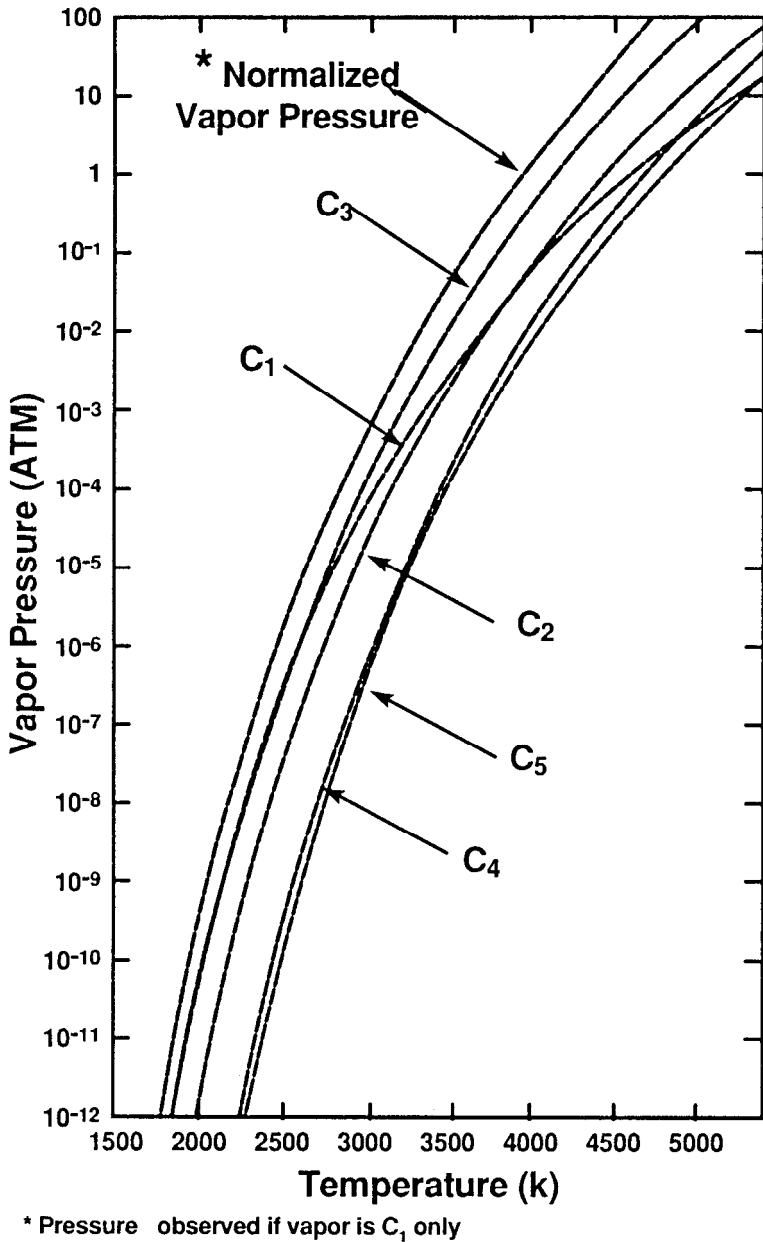
Figure 2.19. Vapor pressure of carbon species.
