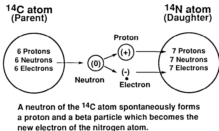
Figure 2.3. Decay of the ^{14}\text{C} radioactive carbon isotope. [8]
