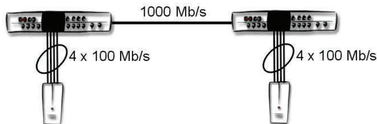
Figure 3. Switch-to-station connection
