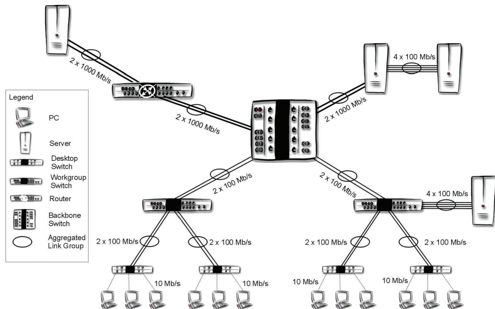
Figure 1. Aggregated links
