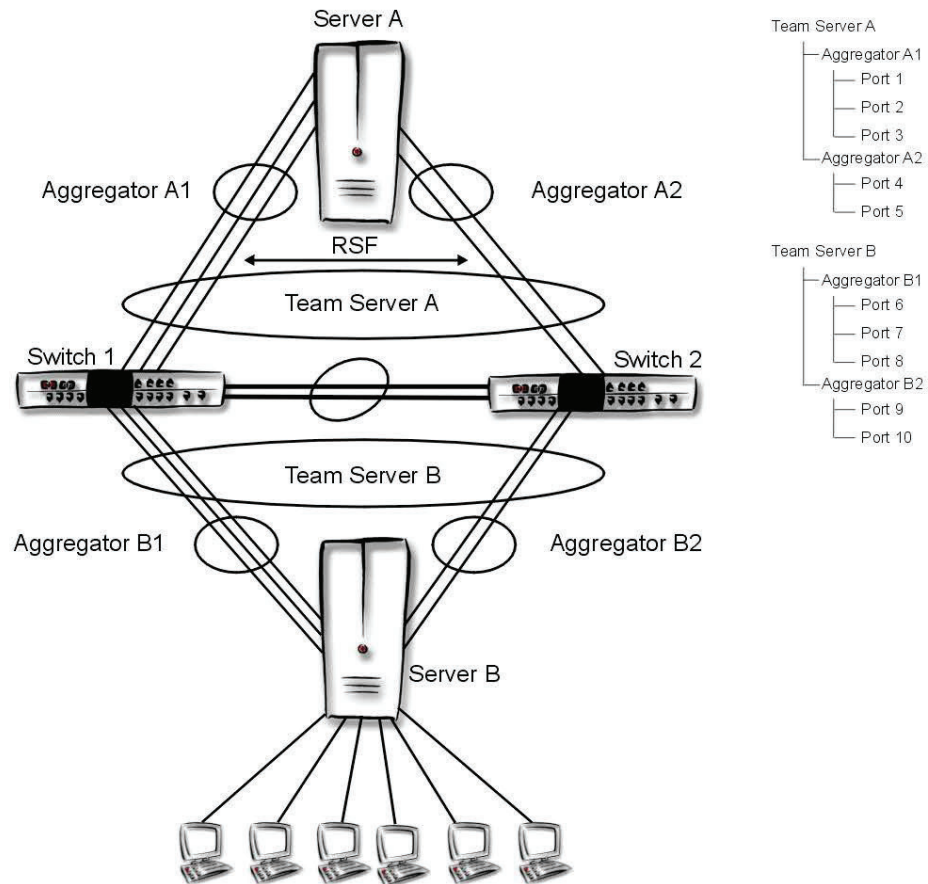
Figure 5. Link Aggregation and RSF
