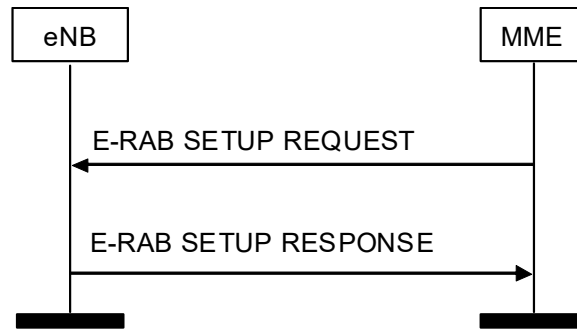
Figure 8.2.1.2-1: E-RAB Setup procedure. Successful operation.
