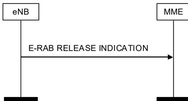
Figure 8.2.3.2.2-1: E-RAB Release INDICATION procedure. Successful operation.
