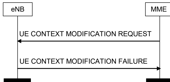
Figure 8.3.4.3-1: UE Context Modification procedure. Unsuccessful operation.
