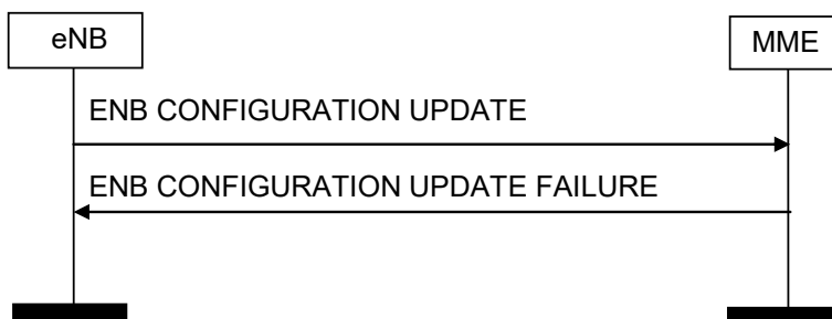
Figure 8.7.4.3-1: ENB Configuration Update procedure: Unsuccessful Operation.
