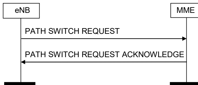
Figure 8.4.4.2-1: Path switch request: successful operation
