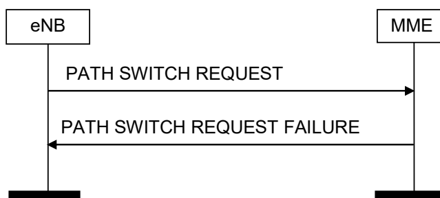
Figure 8.4.4.3-1: Path switch request: unsuccessful operation
