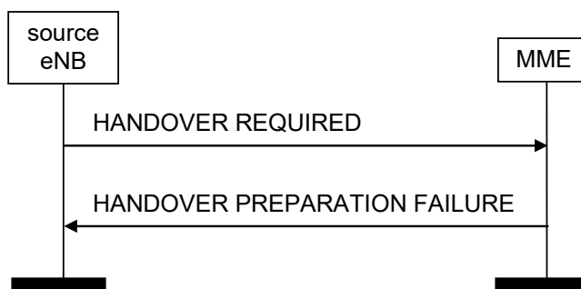
Figure 8.4.1.3-1: Handover preparation: unsuccessful operation
