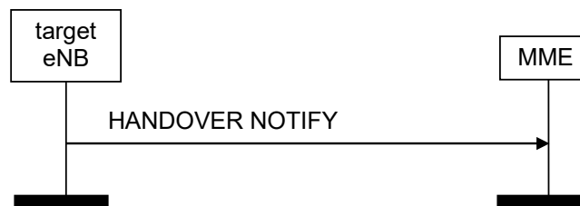
Figure 8.4.3.2-1: Handover notification
