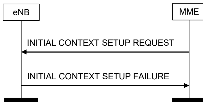
Figure 8.3.1.3-1: Initial Context Setup procedure. Unsuccessful operation.
