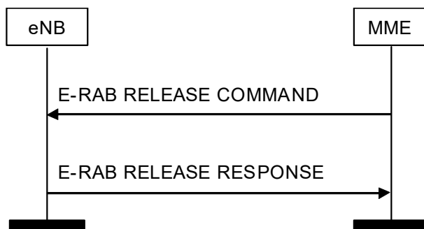
Figure 8.2.3.2.1-1: E-RAB Release procedure. Successful operation.
