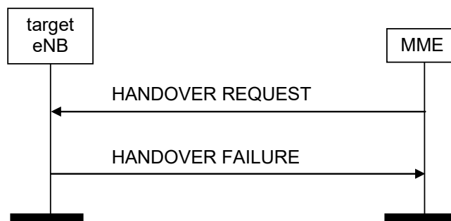
Figure 8.4.2.3-1: Handover resource allocation: unsuccessful operation
