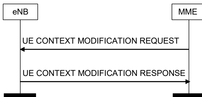
Figure 8.3.4.2-1: UE Context Modification procedure. Successful operation.
