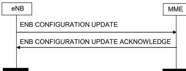
Figure 8.7.4.2-1: ENB Configuration Update procedure: Successful Operation.
