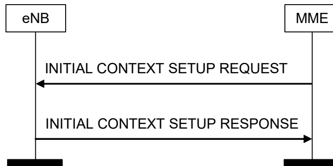
Figure 8.3.1.2-1: Initial Context Setup procedure. Successful operation.
