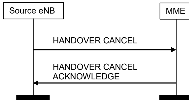
Figure 8.4.5.2-1: Handover Cancel procedure. Successful operation.
