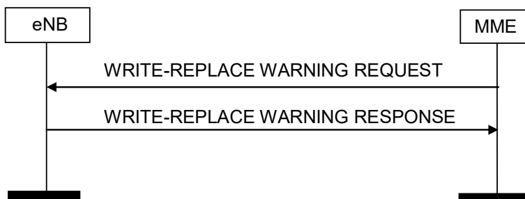
Figure 8.12.1.2-1: Write-Replace Warning procedure. Successful operation.
