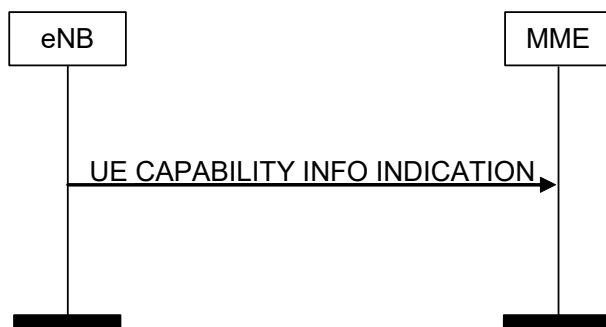
Figure 8.9.2-1: UE Capability Info Indication procedure. Successful operation.
