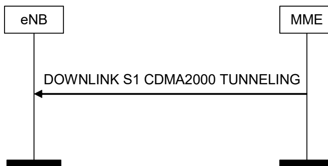
Figure 8.8.2.1-1: Downlink S1 CDMA2000 Tunneling Procedure
