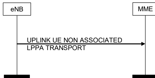
Figure 8.17.2.4-1: UPLINK NON UE ASSOCIATED LPPA TRANSPORT Procedure
