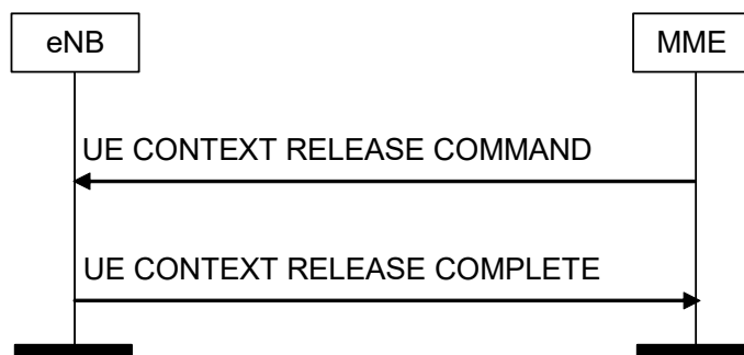
Figure 8.3.3.2-1: UE Context Release procedure. Successful operation.
