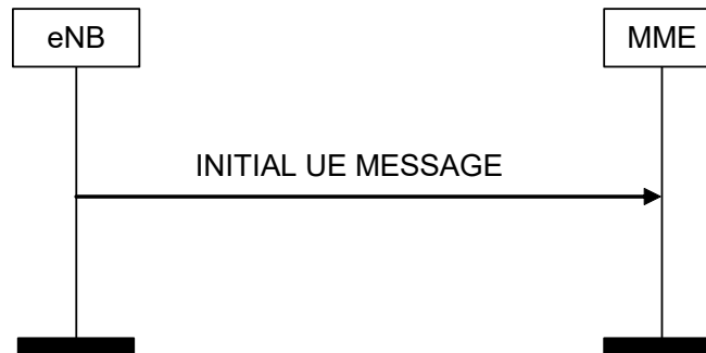
Figure 8.6.2.1-1: Initial UE Message procedure
