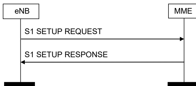
Figure 8.7.3.2-1: S1 Setup procedure: Successful Operation.
