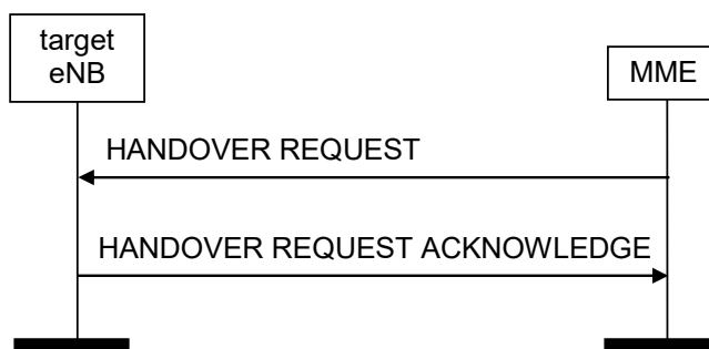
Figure 8.4.2.2-1: Handover resource allocation: successful operation
