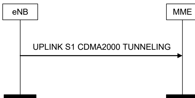
Figure 8.8.2.2-1: Uplink S1 CDMA2000 Tunneling Procedure
