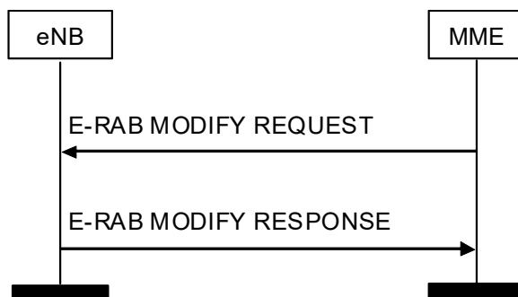
Figure 8.2.2.2-1: E-RAB Modify procedure. Successful operation.
