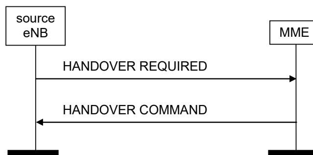
Figure 8.4.1.2-1: Handover preparation: successful operation
