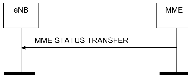
Figure 8.4.7.2-1: MME Status Transfer procedure
