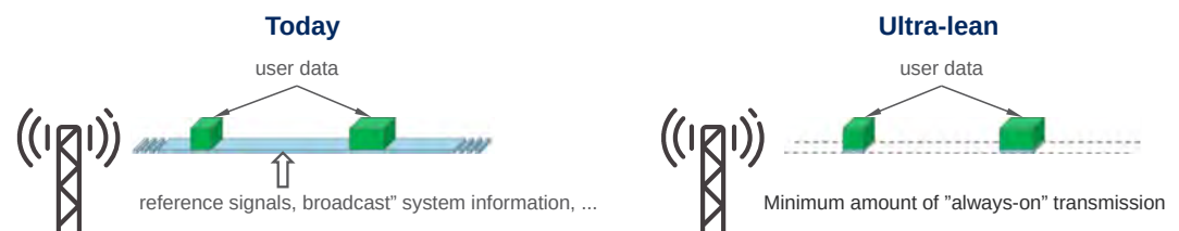
FIGURE 24.1 Ultra-lean transmission.
