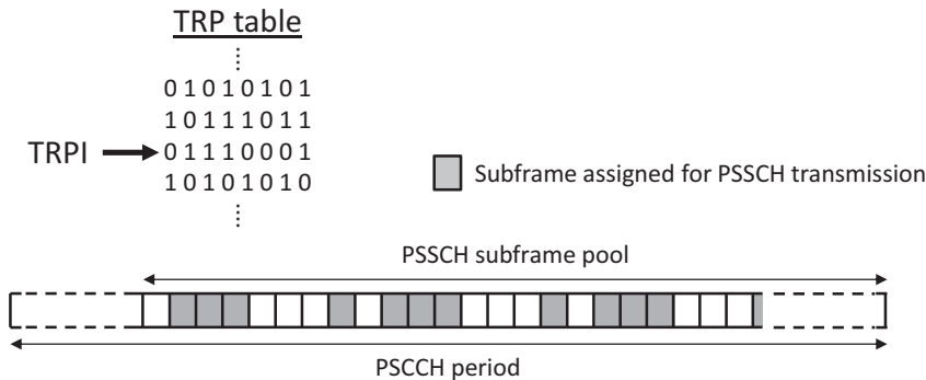
FIGURE 21.11 Assignment of subframes to PSSCH (sidelink communication mode 1).
