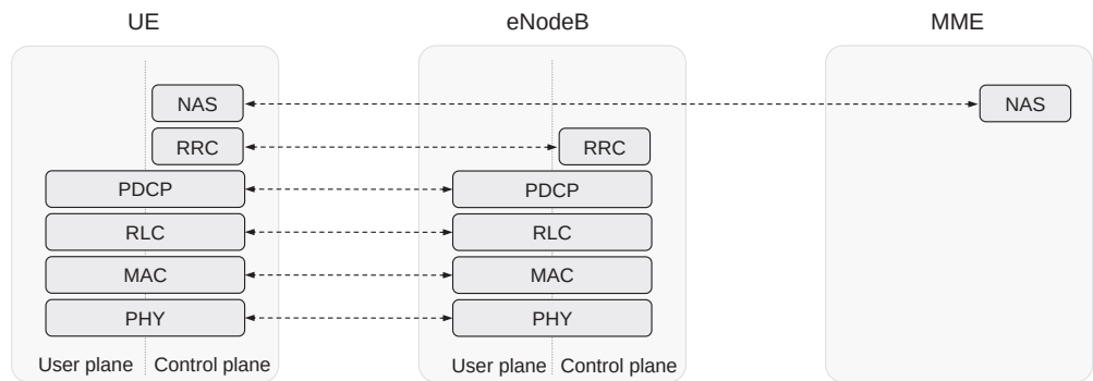
FIGURE 4.3 Overall RAN protocol architecture.
