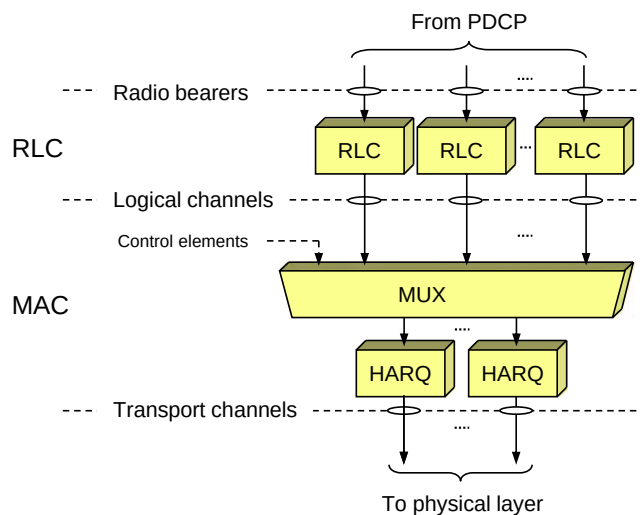
FIGURE 12.4 RLC and hybrid-ARQ retransmission mechanisms in LTE.
