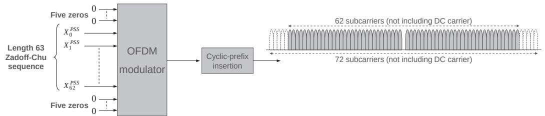
FIGURE 11.2 Definition and structure of PSS.
