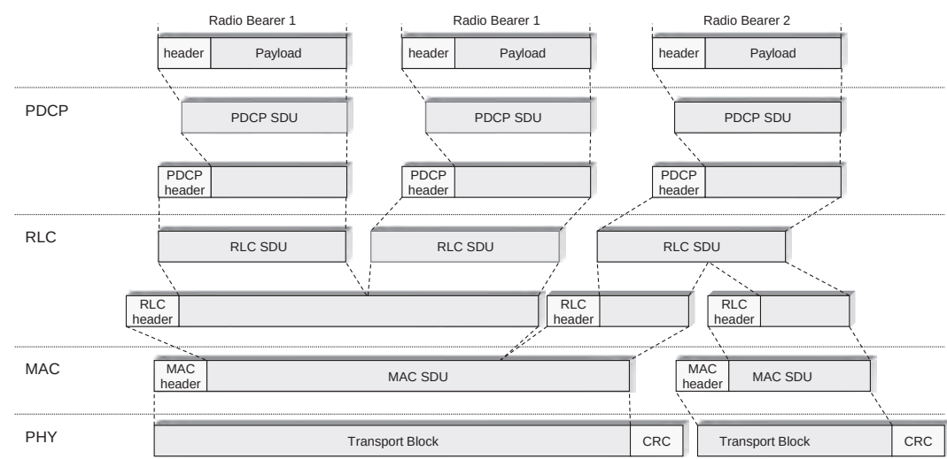
FIGURE 4.5 Example of LTE data flow.
