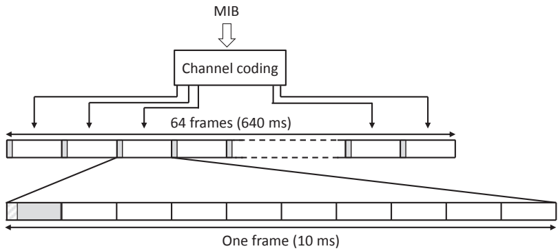
FIGURE 20.12 NB-IoT system information.
