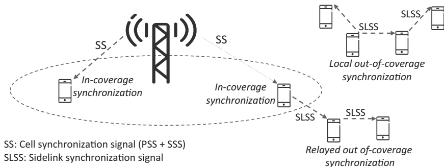
FIGURE 21.3 Transmission-timing acquisition for sidelink transmissions.
