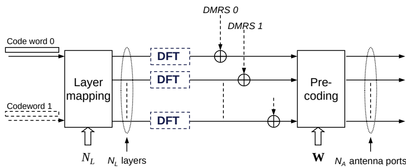
FIGURE 7.18 Precoder-based multi-antenna transmission for LTE uplink.
