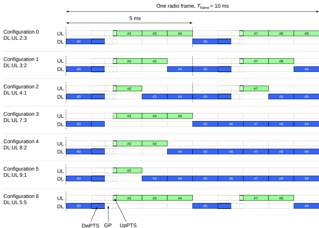
FIGURE 5.7 Different uplink–downlink configurations in case of TDD.
