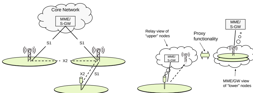
FIGURE 18.3 LTE relaying architecture.
