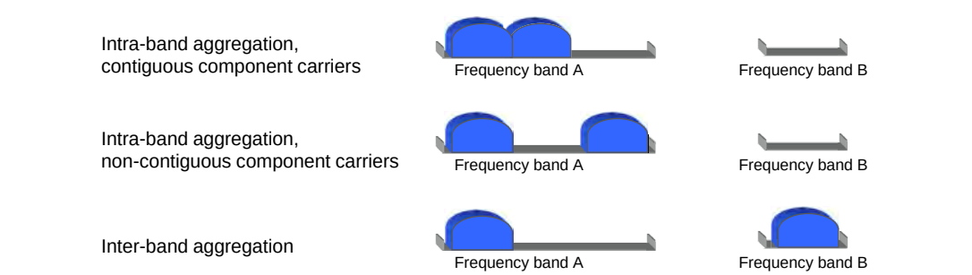
FIGURE 3.6 Carrier aggregation.
