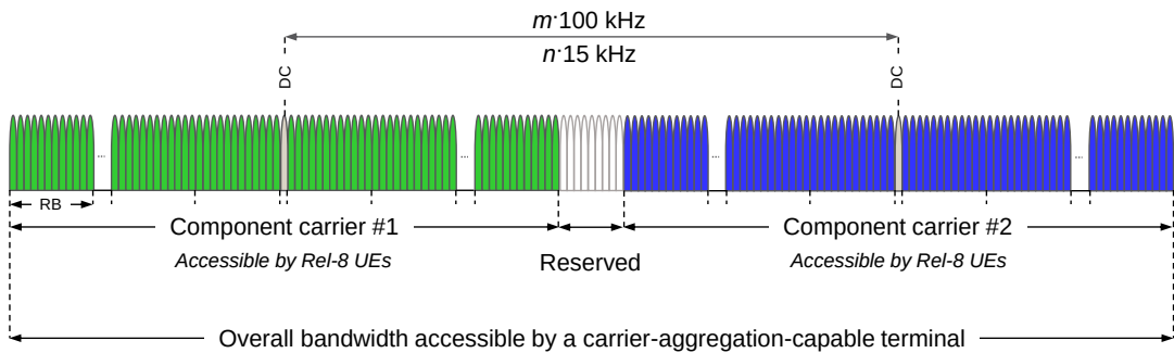
FIGURE 5.11 LTE carrier raster and carrier aggregation.
