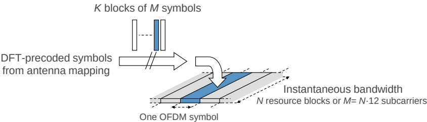
FIGURE 7.3 Mapping to the uplink physical resource.
