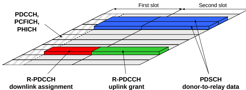
Example of R-PDCCH transmission.
