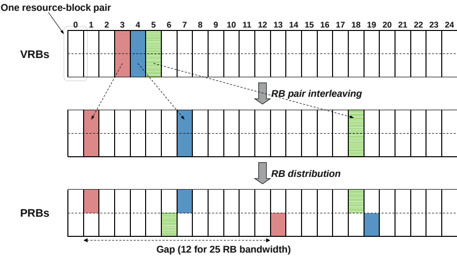
FIGURE 6.7 VRB-to-PRB mapping in case of distributed VRBs. Figure assumes a cell bandwidth corresponding to 25 resource blocks.
