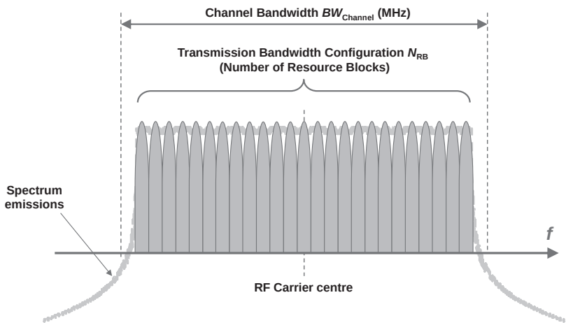
FIGURE 22.2 The channel bandwidth for one RF carrier and the corresponding transmission bandwidth configuration.
