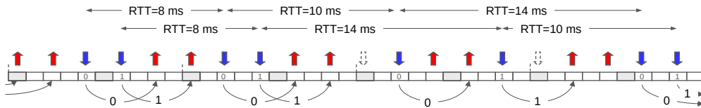
Example of hybrid-ARQ process numbering for FDD.
