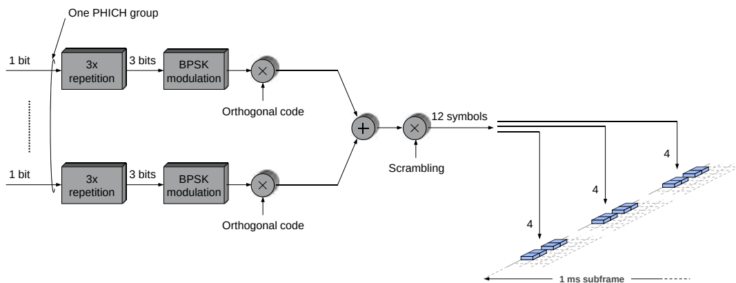
FIGURE 6.24 PHICH structure.
