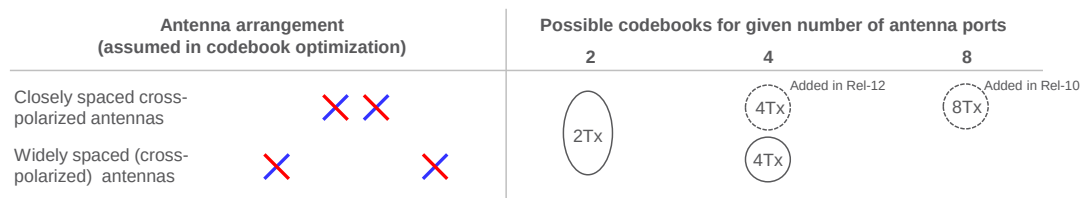
FIGURE 10.1 Assumptions on antenna arrangements for different codebooks.
