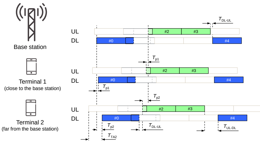
Timing relation for TDD operation.
