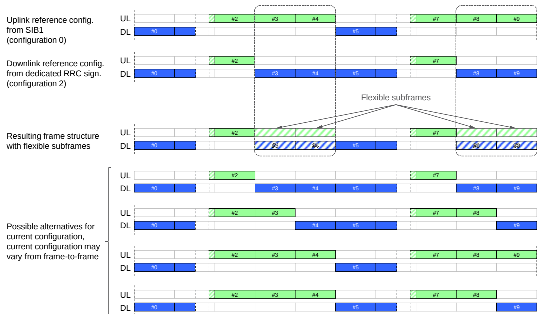
FIGURE 15.3 Example of flexible subframes.
