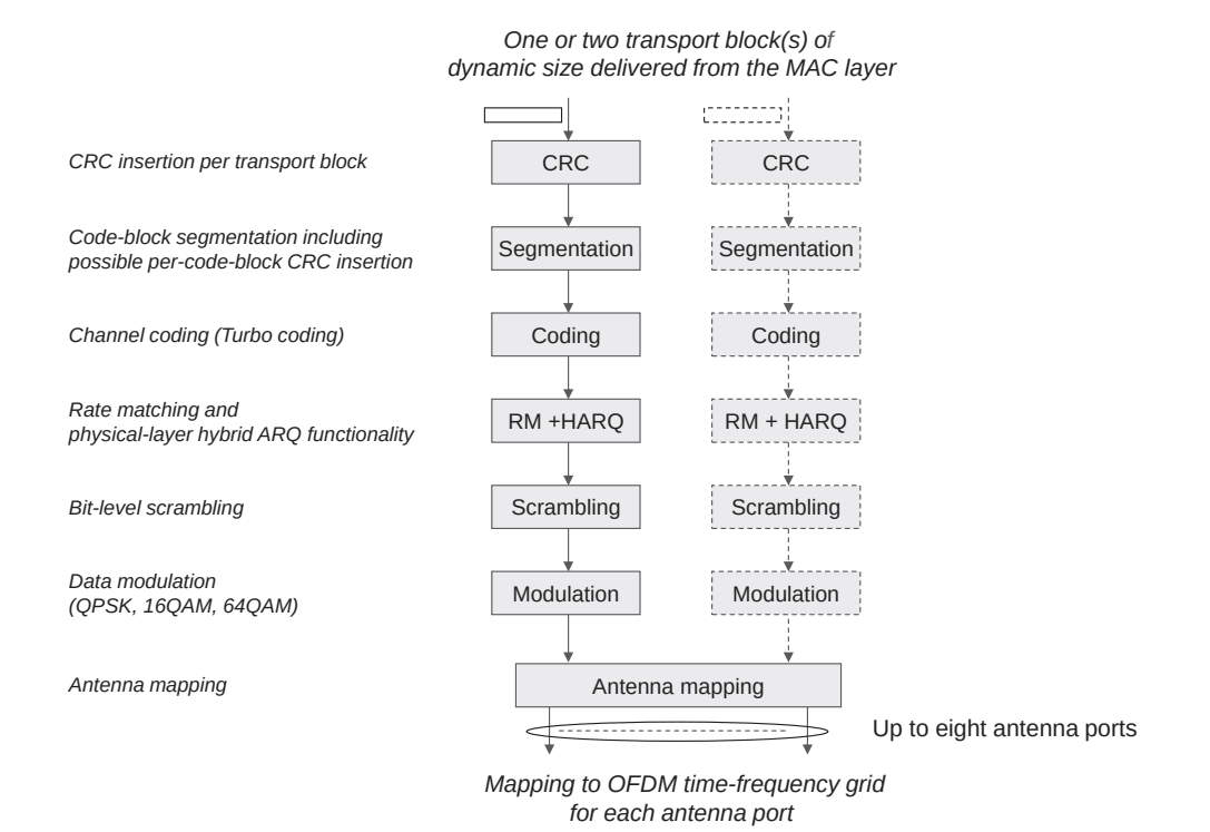
FIGURE 6.1 Physical-layer processing for the downlink shared channel (DL-SCH).
