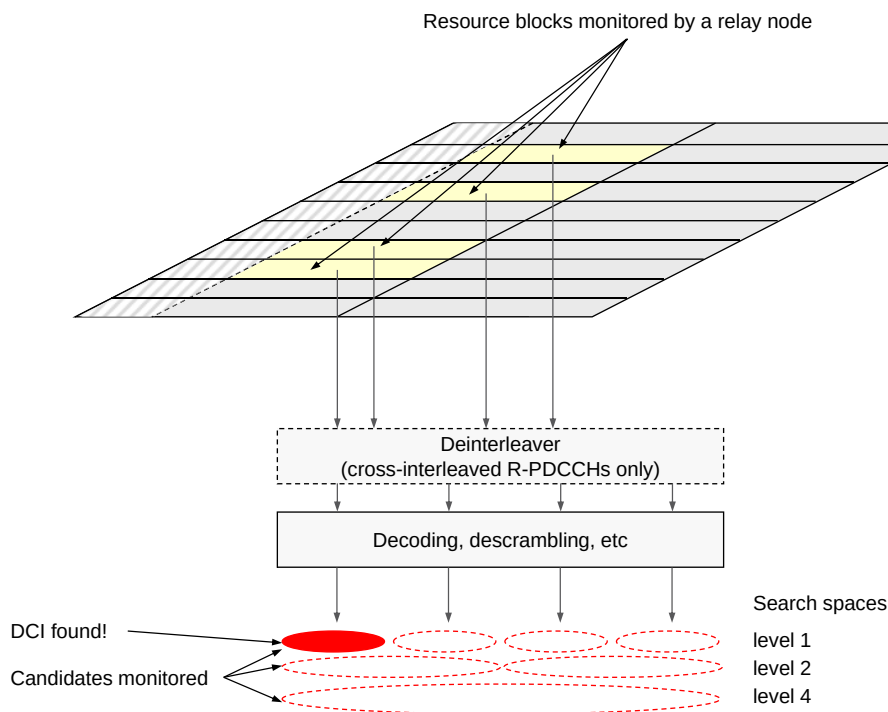
FIGURE 18.9 Principle illustration of R-PDCCH monitoring.
