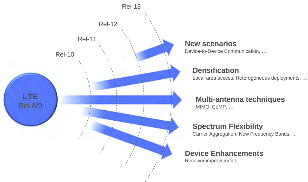
FIGURE 3.5 LTE evolution.
