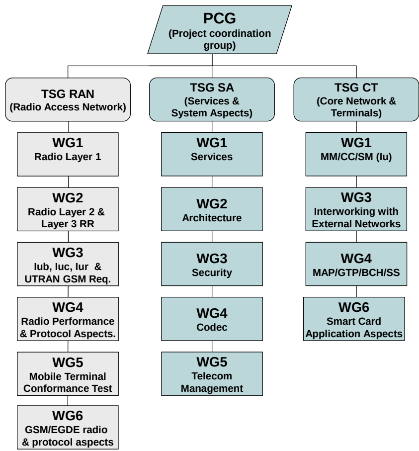
FIGURE 2.9 3GPP organization.
