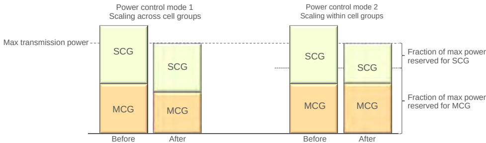
FIGURE 16.7 Power-control behavior for mode 1 and 2 when reaching the maximum transmission power.
