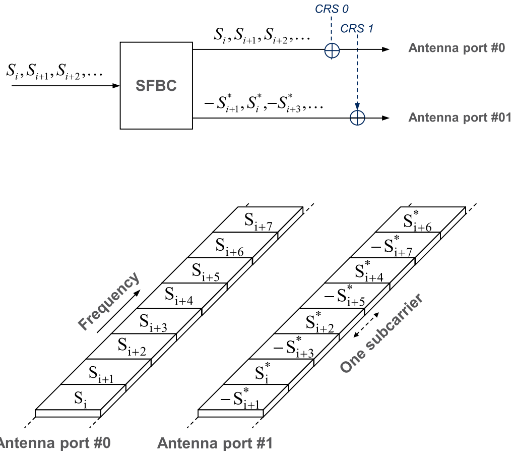
FIGURE 6.15 Transmit diversity for two antenna ports—SFBC.
