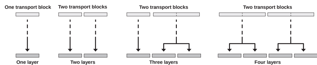
FIGURE 7.19 Uplink transport-channel-to-layer mapping (initial transmission).
