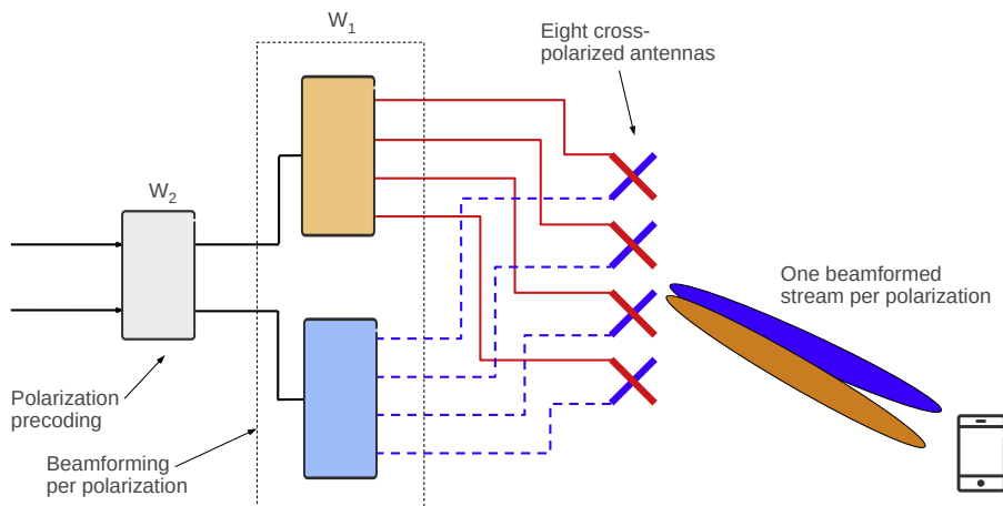
FIGURE 10.2 Illustration of the eight-antenna codebook.
