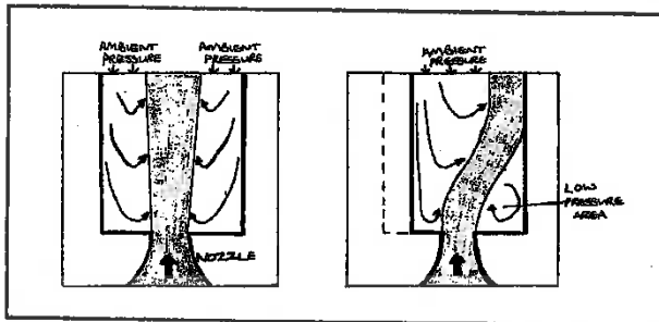
Figure 1. The Coanda effect. (Image by Caroline Lubert, based on image from Scientific American , December 1964, pages 80–88).
