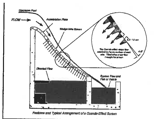
Figure 5. Operating principles of a Coanda stormwater filtration screen. (Image taken from Wahl, Tony L., 2003, Design Guidance for Coanda-Effect Screens . U.S. Dept. of the Interior, Bureau of Reclamation, Research Report R-03-03. July 2003. [online paper]).
