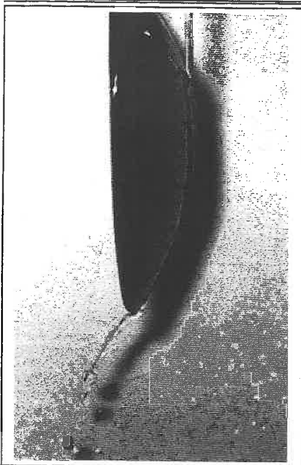
Figure 2. The Teapot effect (Image by Axda0002 at en.wikipedia [CC-BY-SA-2.5 ( www.creativecommons.org/licenses/by-sa/2.5 )], via Wikimedia Commons).
